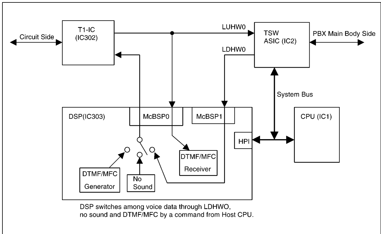
Fig. 5.4 Image View of the DSP (IC303) Internal Processing
