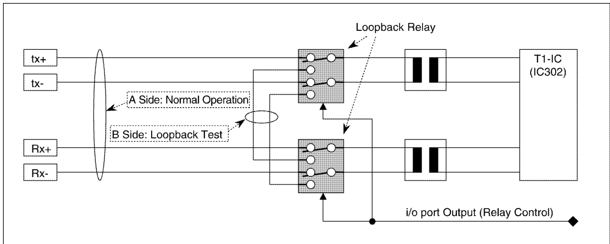
Fig.5.3 Outline diagram of the line interface
