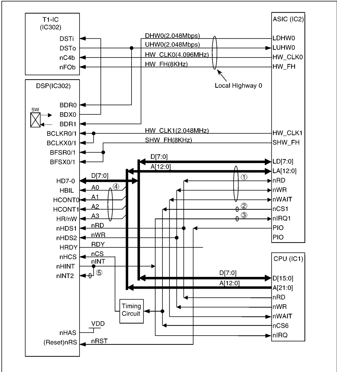
Fig.5.5 New PBX...DSP (IC303) Signal Line Connection Diagram
