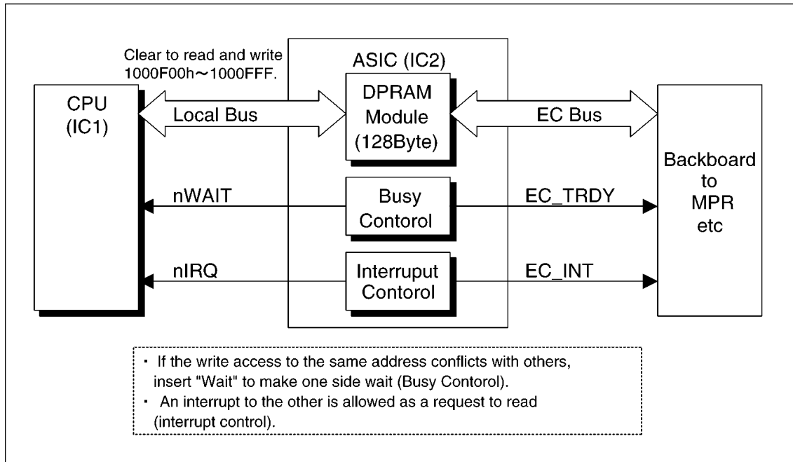
Fig.5.7 DPRAM Communication diagrammatic illustration
