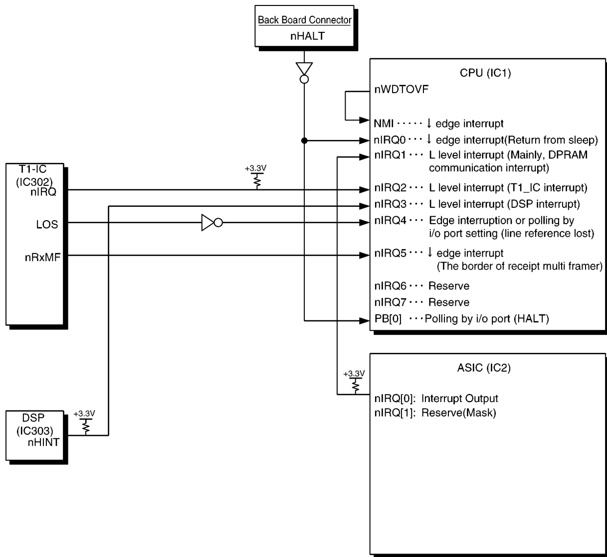
Fig.5.1 External interrupt image
