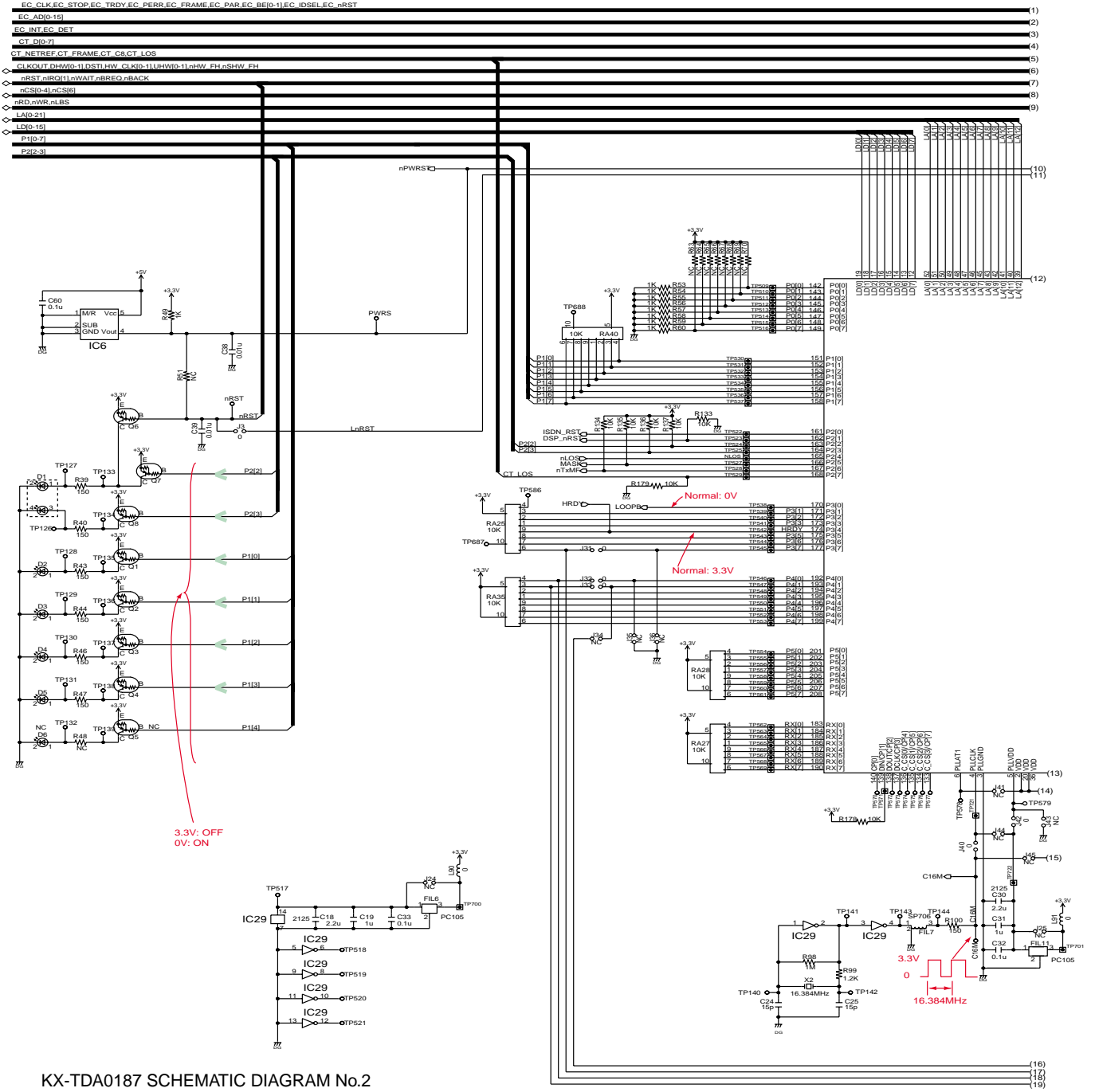
KX-TDA0187 SCHEMATIC DIAGRAM No.2
