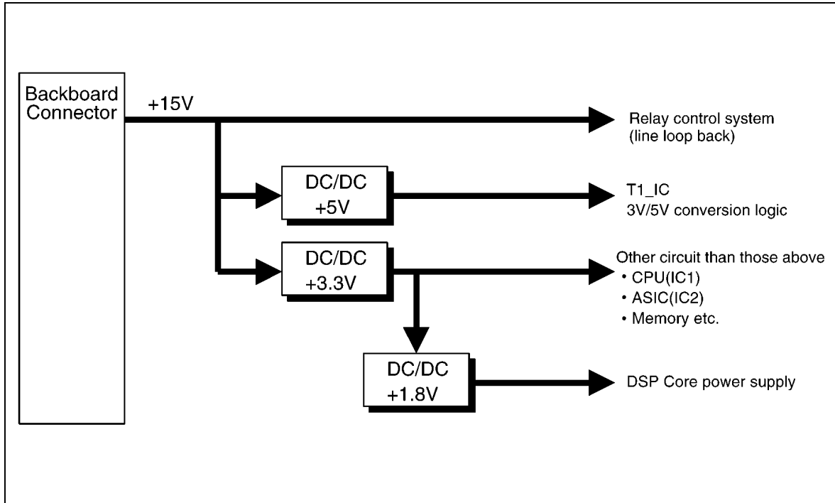
Fig.5.9 System diagram of the power supply
