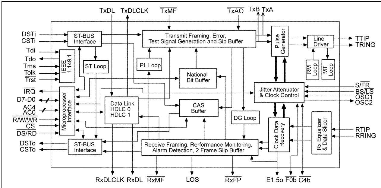
Fig.5.2 Outline block diagram of the T1-IC (IC302)
