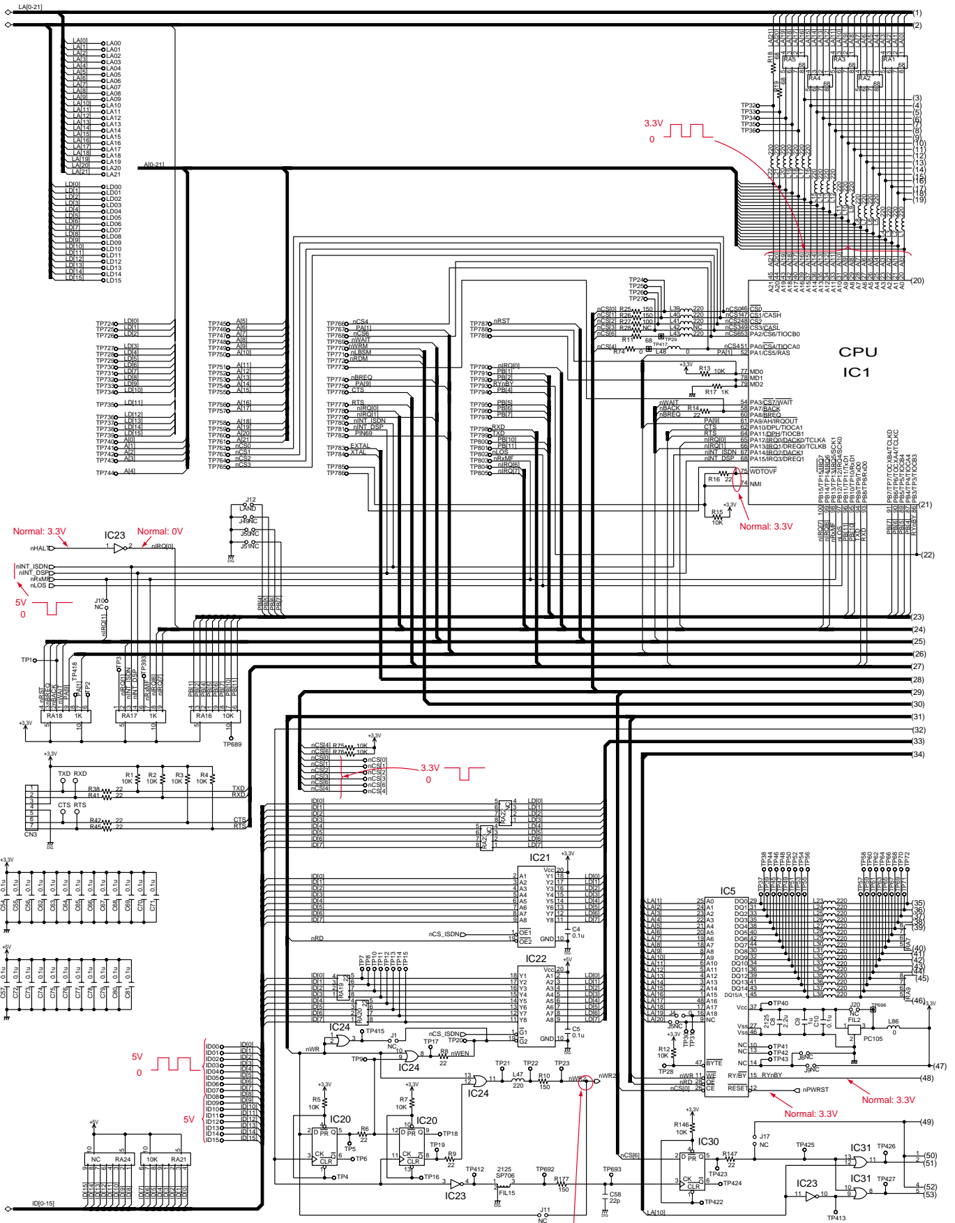
KX-TDA0187 SCHEMATIC DIAGRAM No.1
