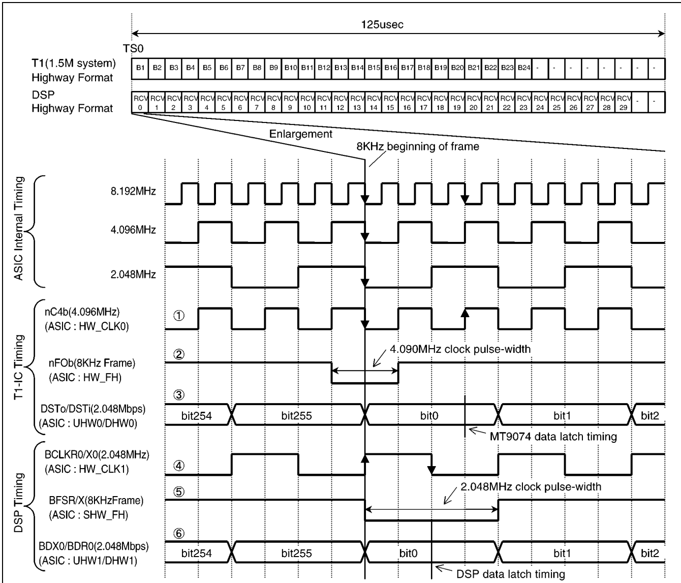
Fig 5.6 Shows the Bch Highway Assignment and the Input/Output Timings of the ASIC (IC2), the T1-IC (IC302) and the DSP (IC303)
