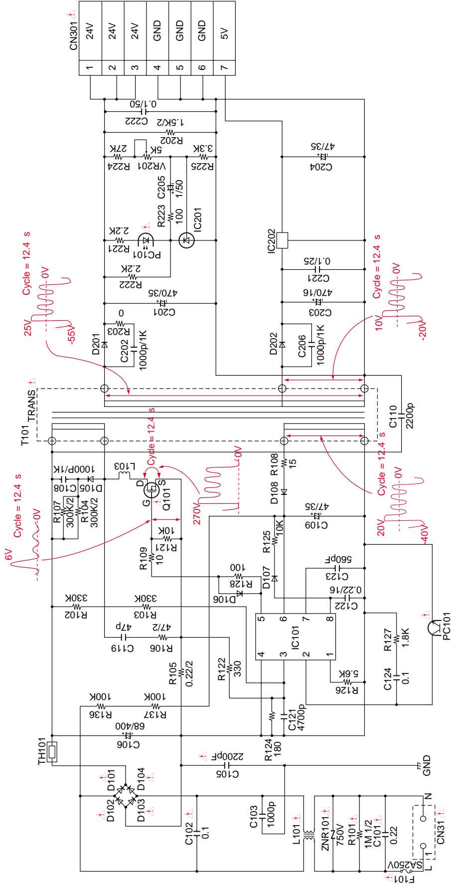
KX-FP342BX : POWER SUPPLY BOARD (PCB4)
