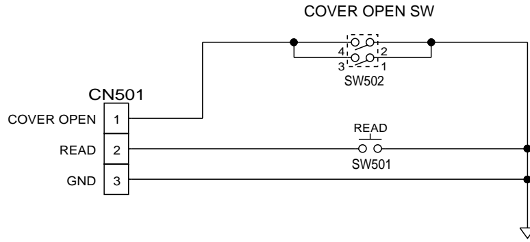
KX-FP342BX : SENSOR BOARD (PCB5)
