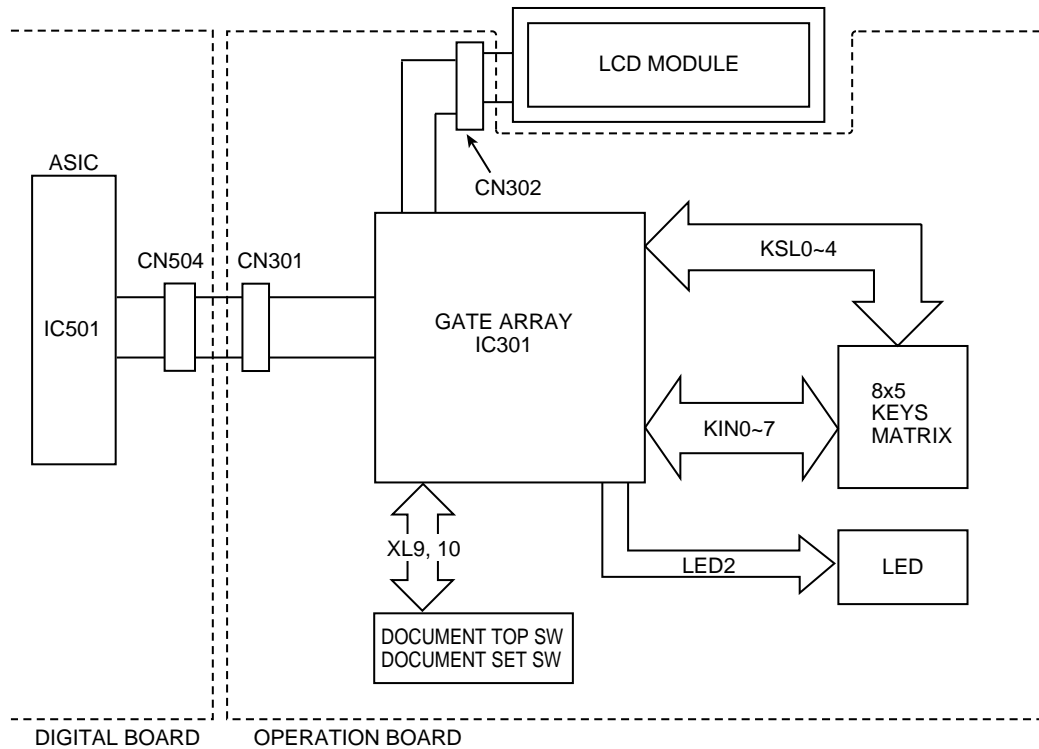
KX-FP342BX:OPERATION BOARD BLOCK DIAGRAM
