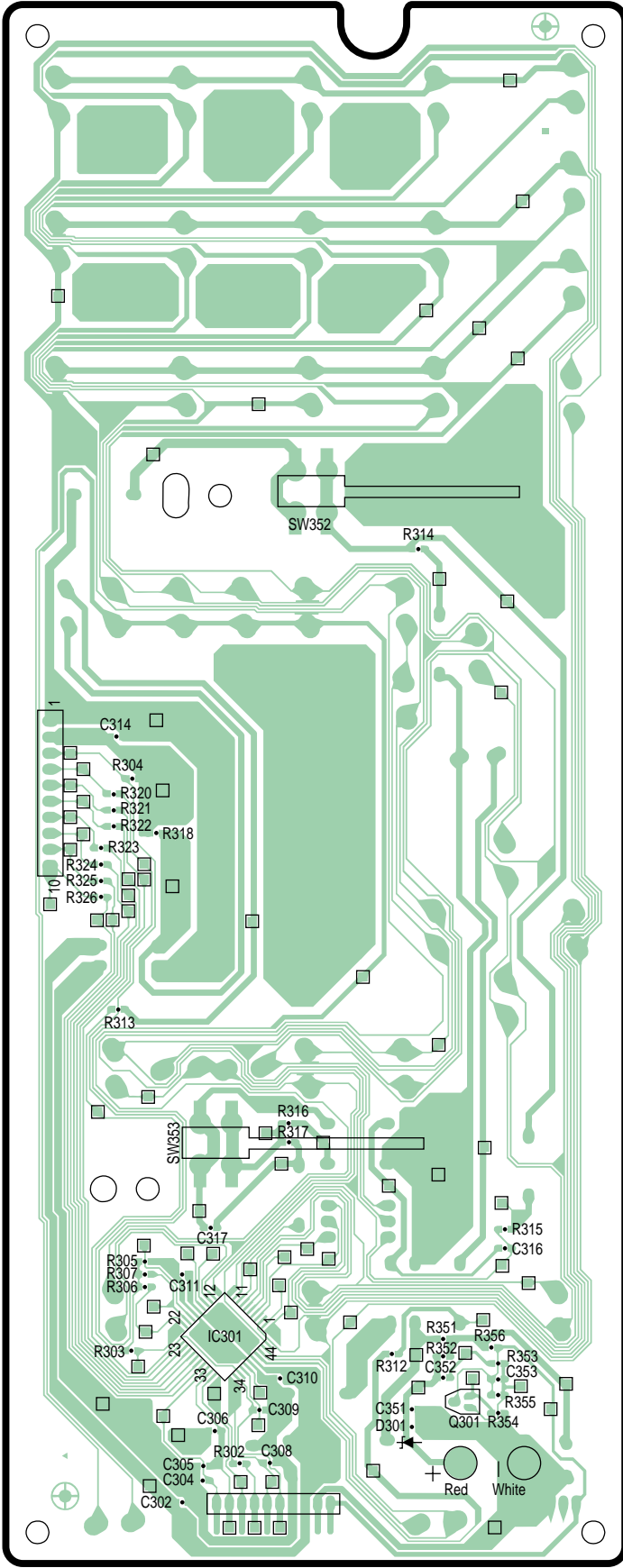
KX-FP342BX : OPERATION BOARD(PCB3) : BOTTOM VIEW
