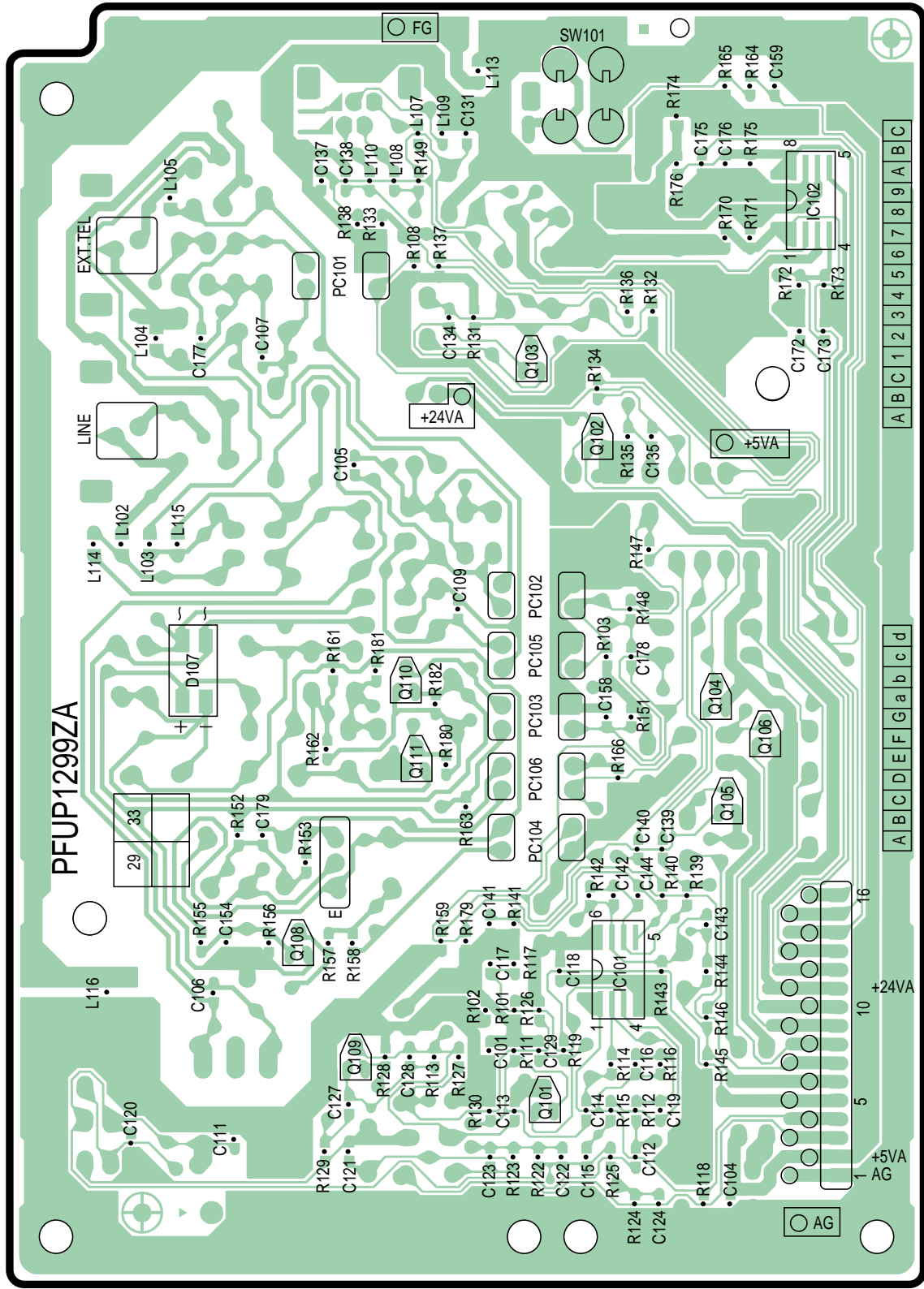
KX-FP342BX : ANALOG BOARD(PCB2) : BOTTOM VIEW
