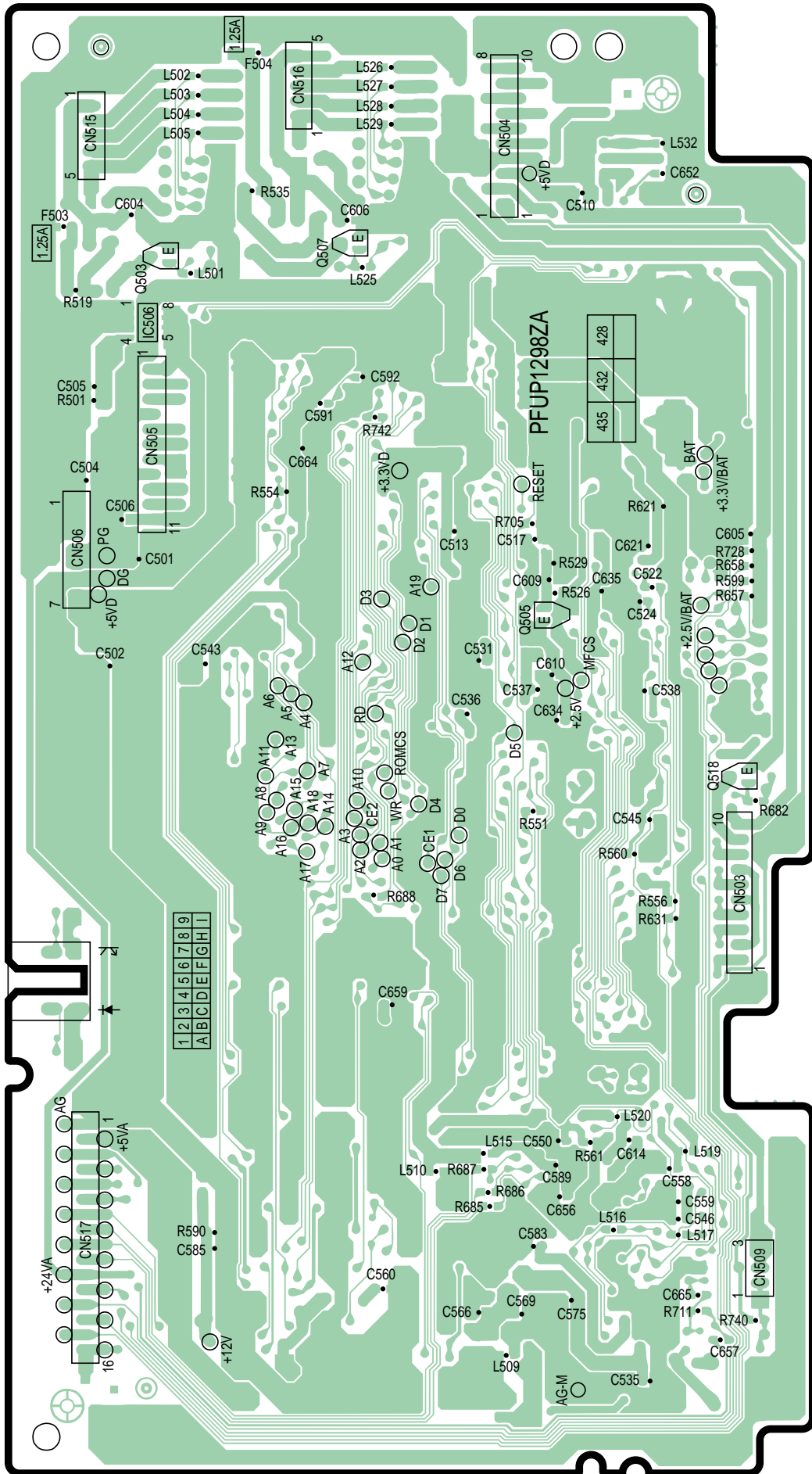
KX-FP342BX : DIGITAL BOARD(PCB1) : BOTTOM VIEW
