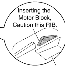
Hook Lever
