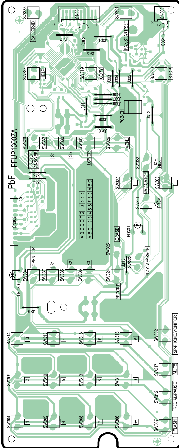
KX-FP342BX : OPERATION BOARD(PCB3) : COMPONENT VIEW
