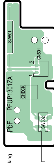
KX-FP342BX : SENSOR BOARD(PCB5)
