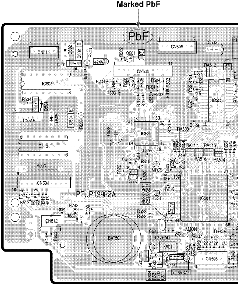
(Digital Board : Component View)
