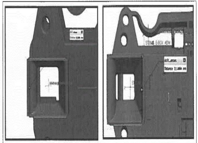
Old door lock design (left) vs New door lock design (right)
