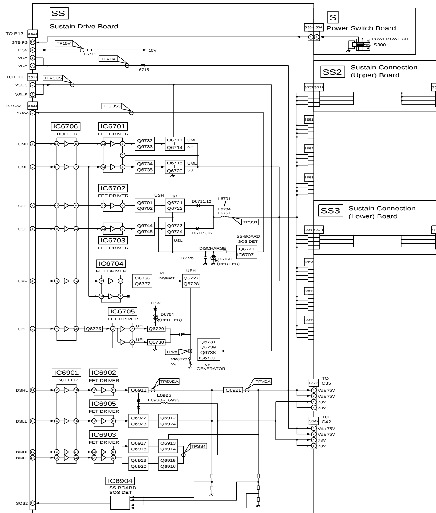
TH-50PV30A/H/M/R SS,S,SS2 and SS3-Board Block Diagram
