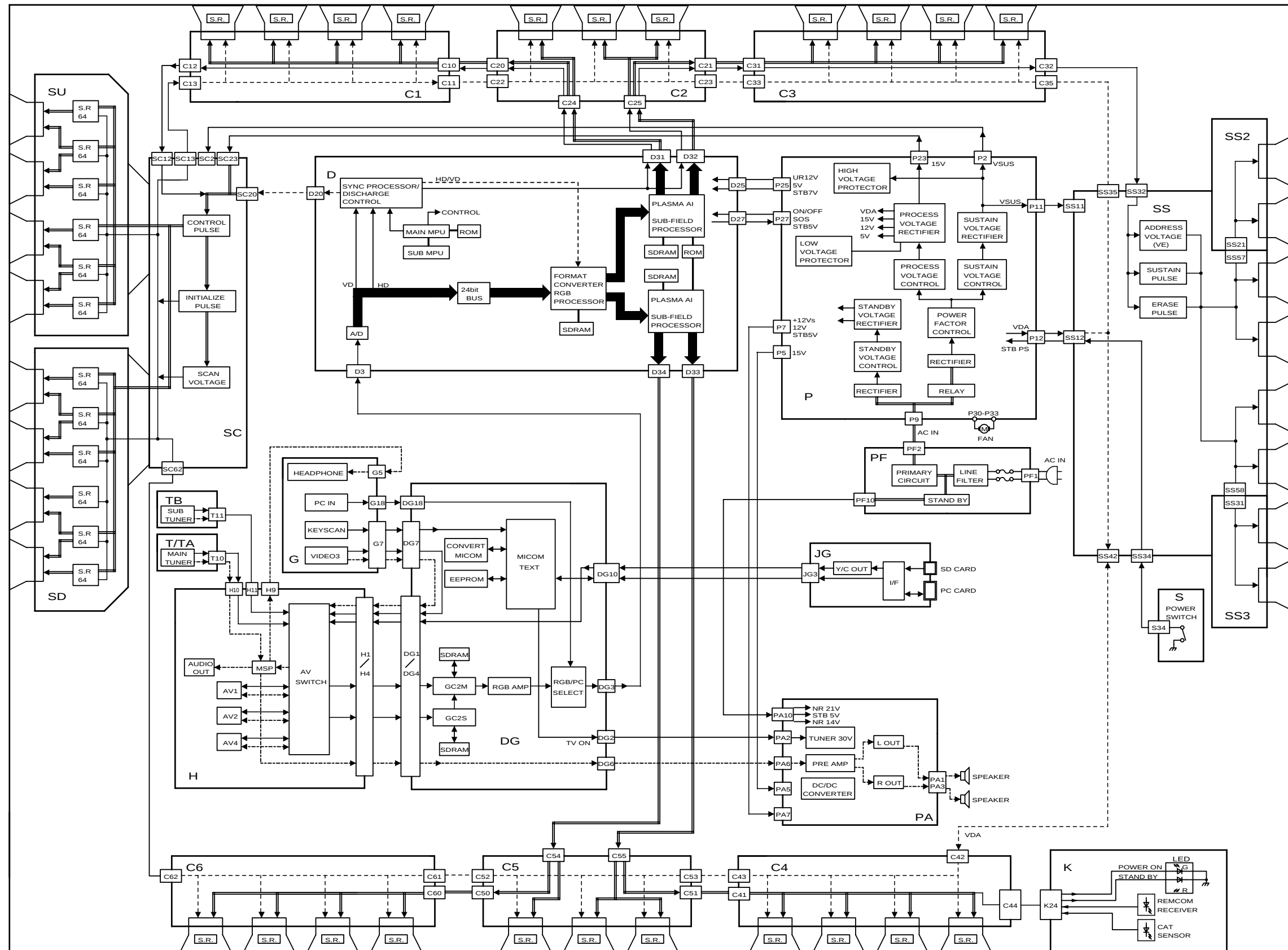
TH-50PV30A/H/M/R Main Block Diagram
