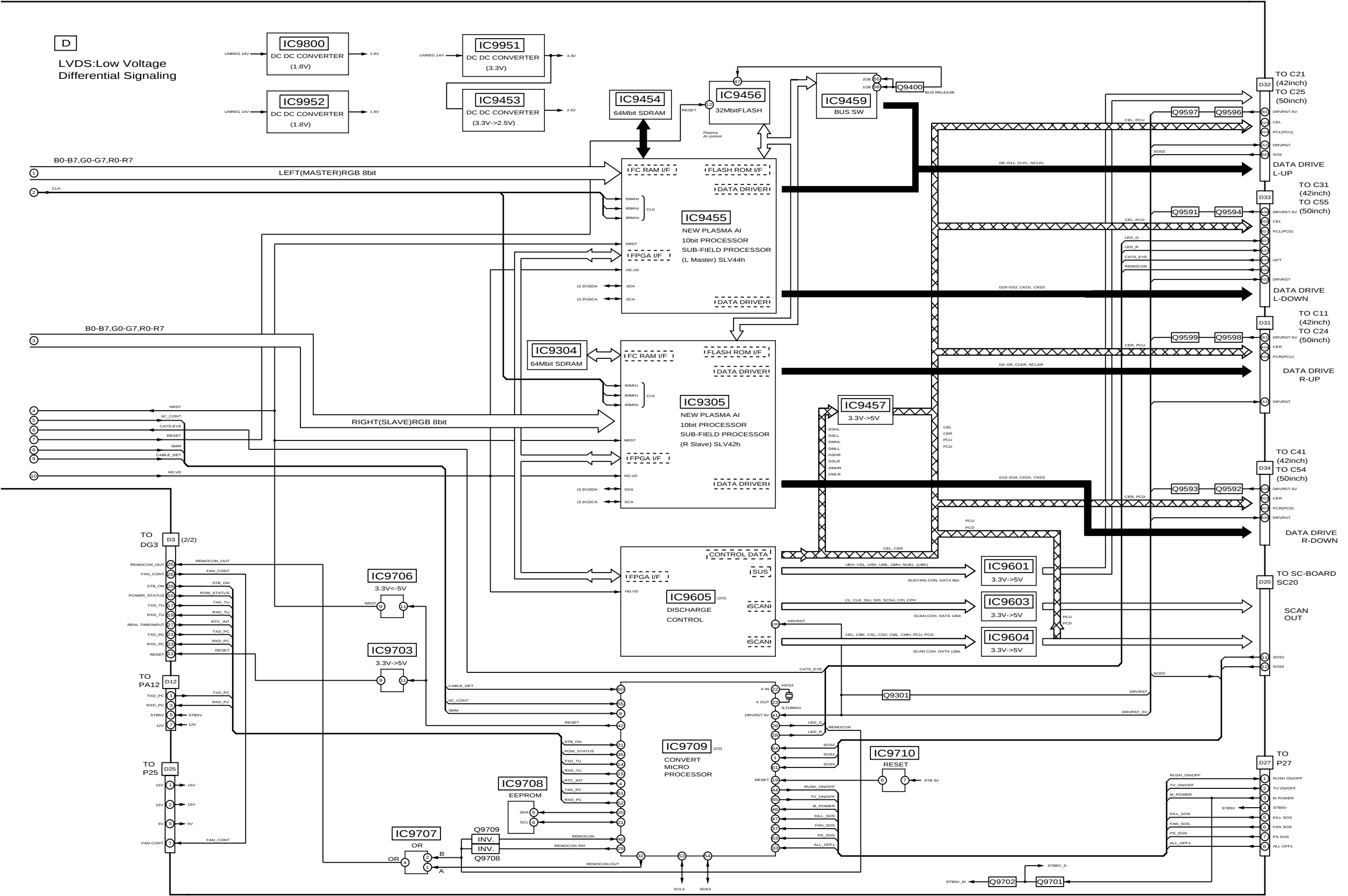
TH-50PV30A/H/M/R D-Board Block Diagram
