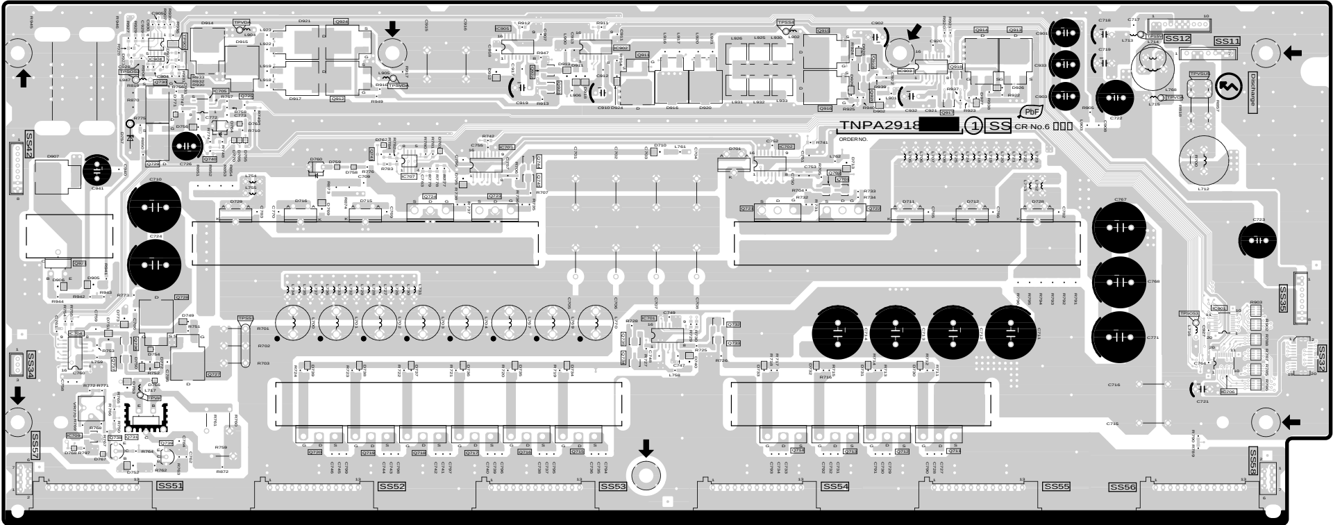
SS-BBOARD (COMPONENT SIDE) TXNSS20RTS
