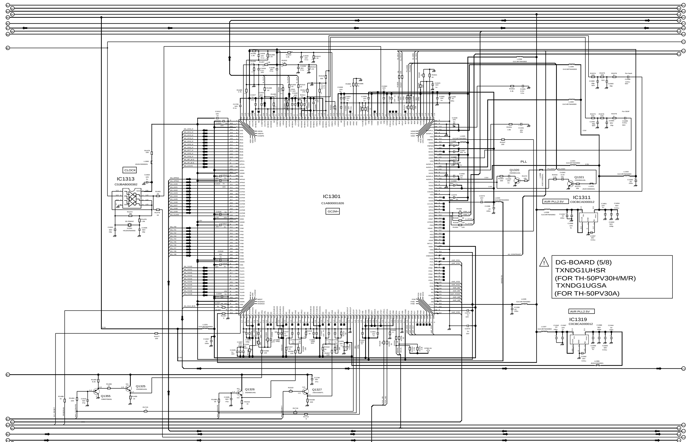
TH-50PV30A/H/M/R DG-Board (5 of 8) Schematic Diagram
