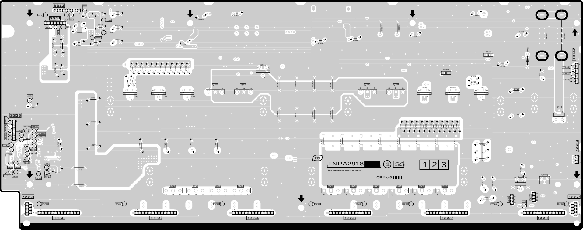
SS-BOARD (FOIL SIDE) TXNSS20RTS
