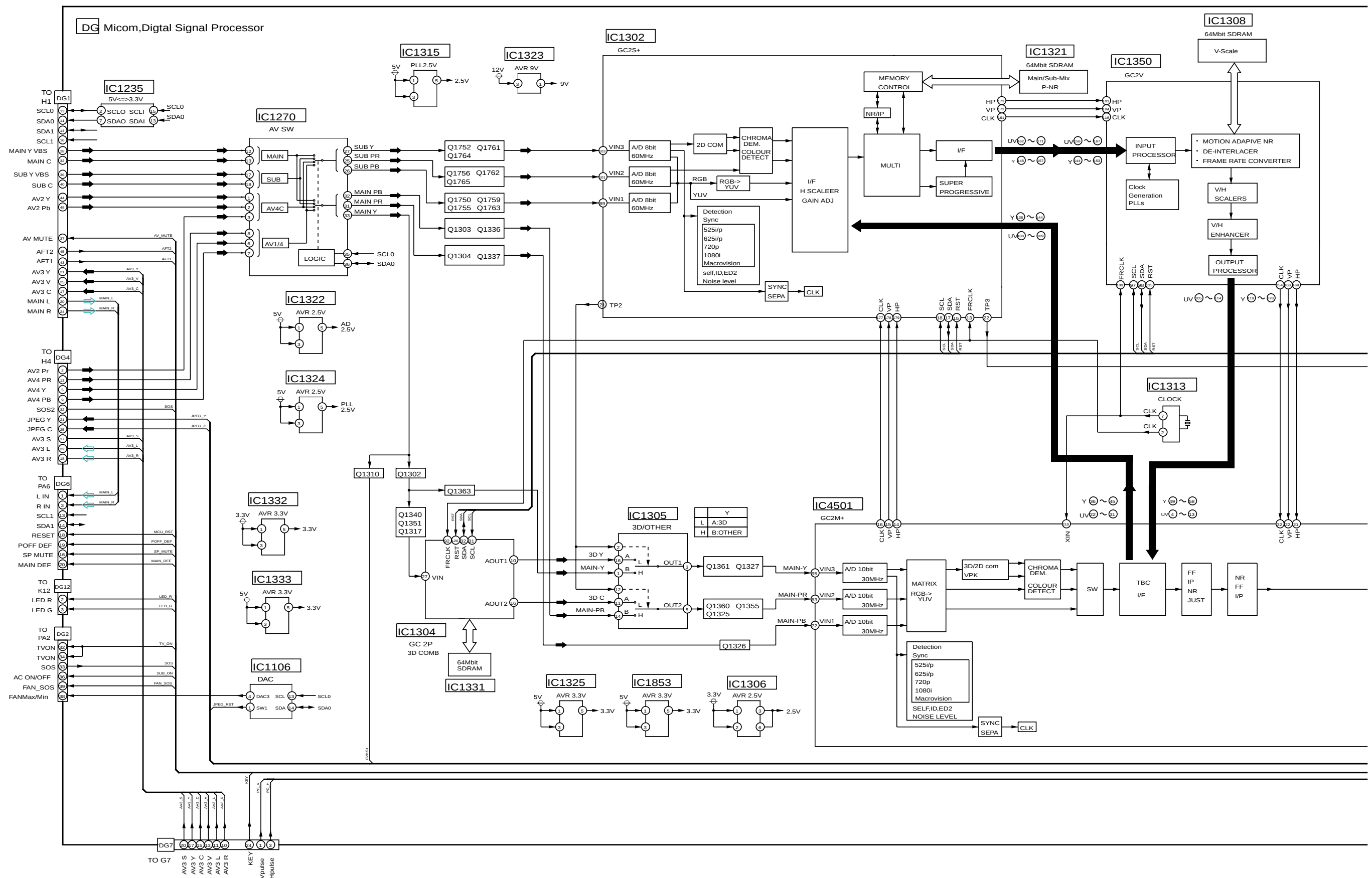
TH-50PV30A/H/M/R DG-Board (1 of 2) Block Diagram
