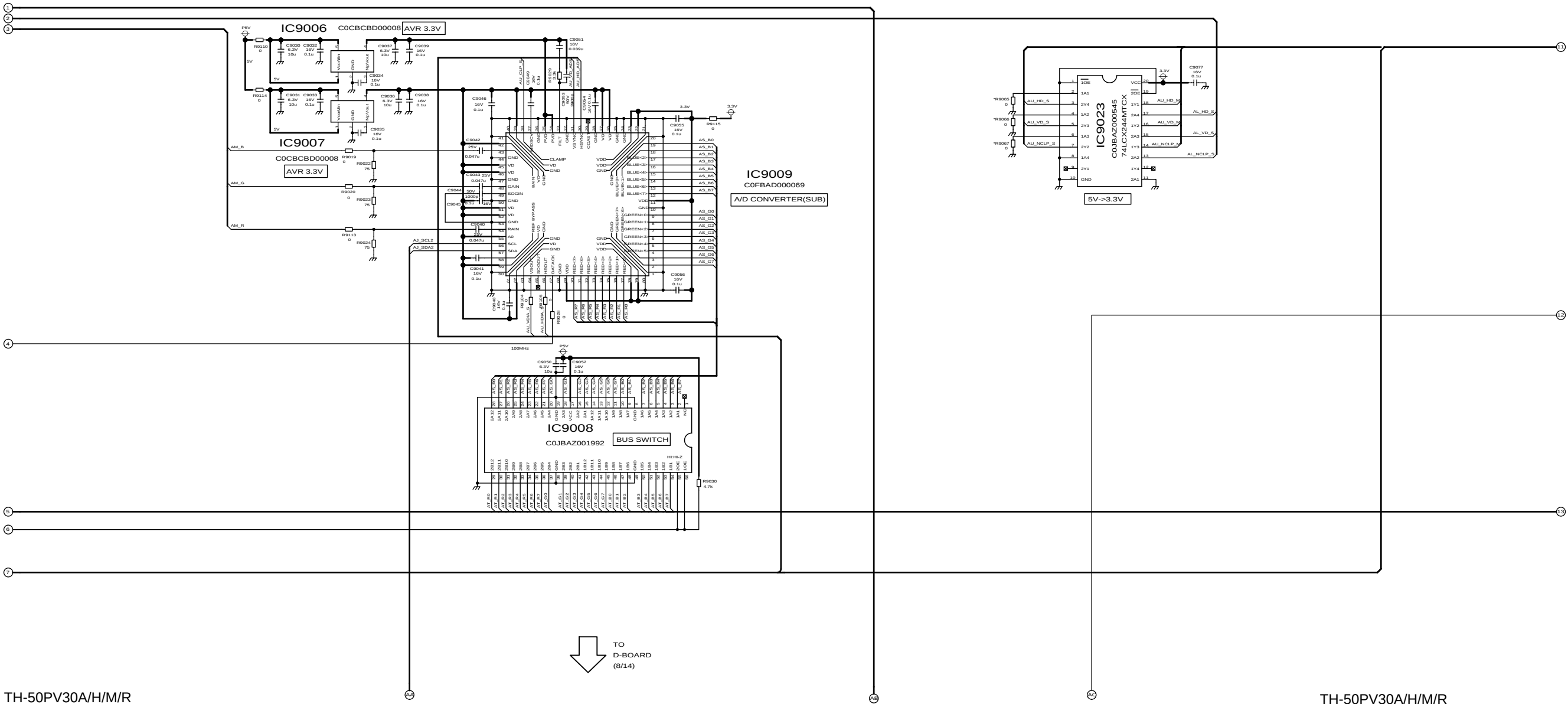
TH-50PV30A/H/M/R D-Board (2 of 14) Schematic Diagram
