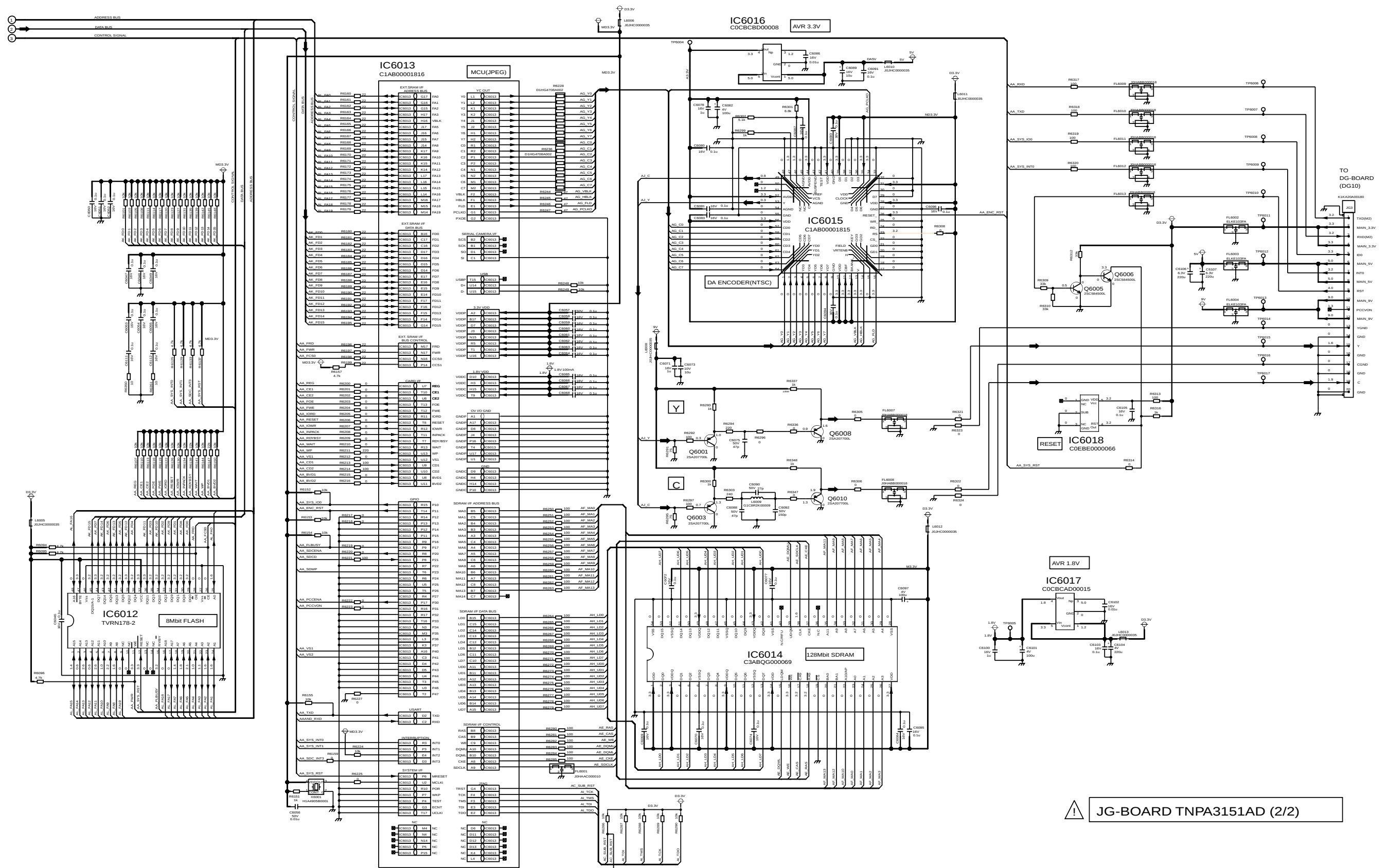
TH-50PV30A/H/M/R JG-Board (2 of 2) Schematic Diagram
