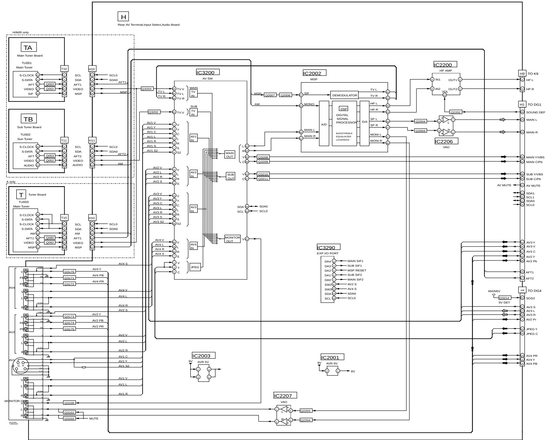
TH-50PV30A/H/M/R H, T, TA, and TB-Board Block Diagram
