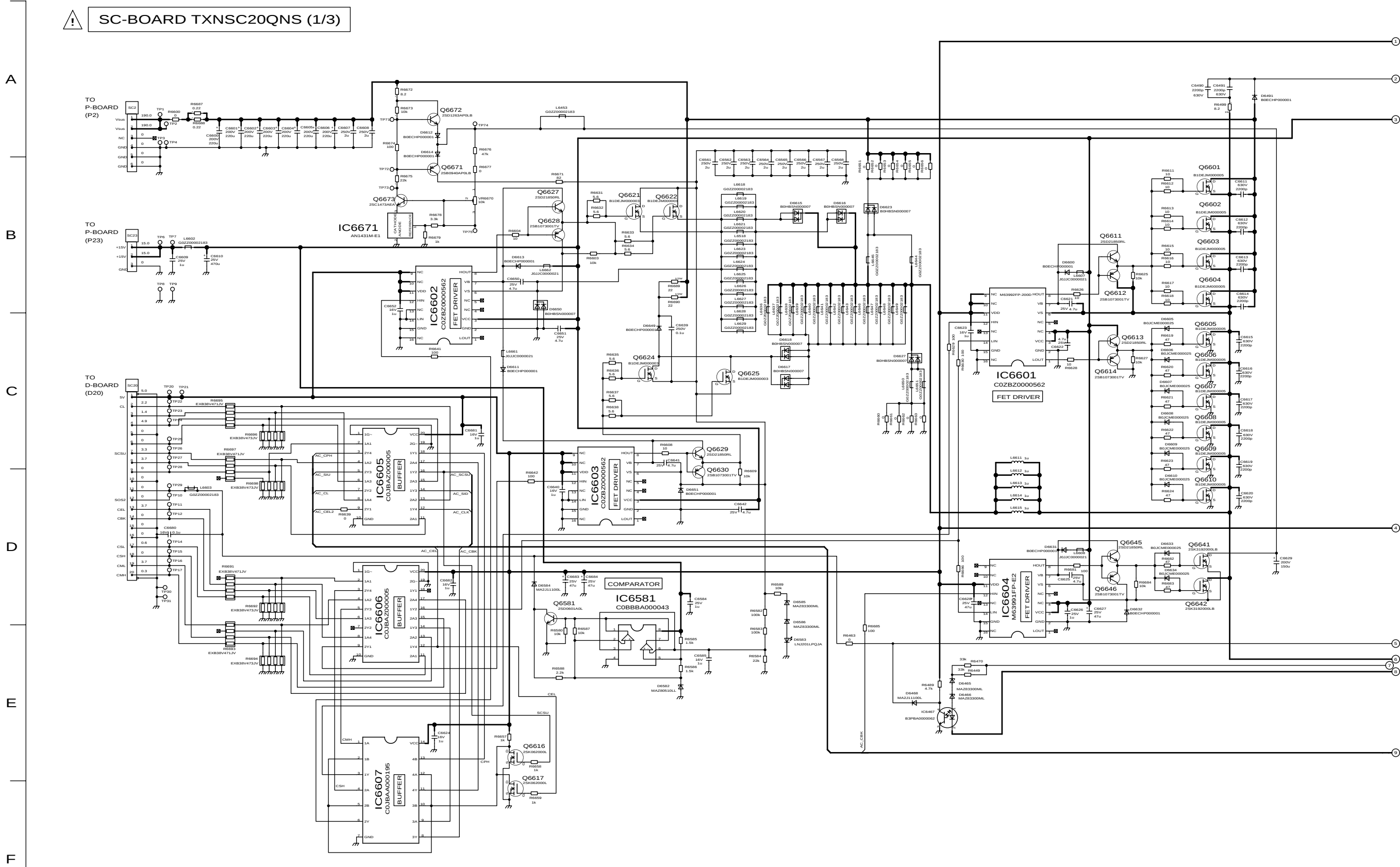
TH-50PV30A/H/M/R SC-Board (1 of 3) Schematic Diagram
