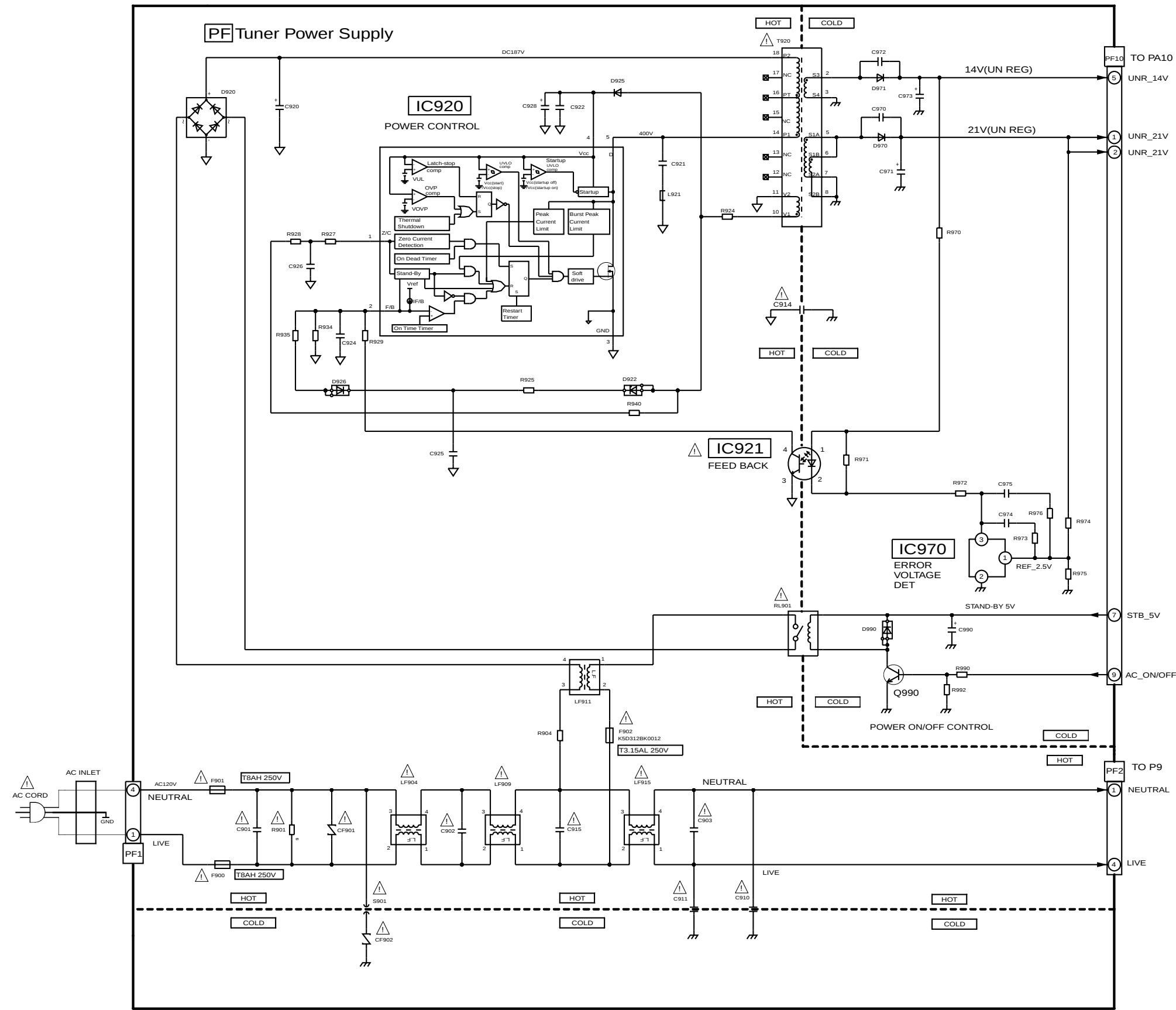
TH-50PV30A/H/M/R PF-Board Block Diagram
