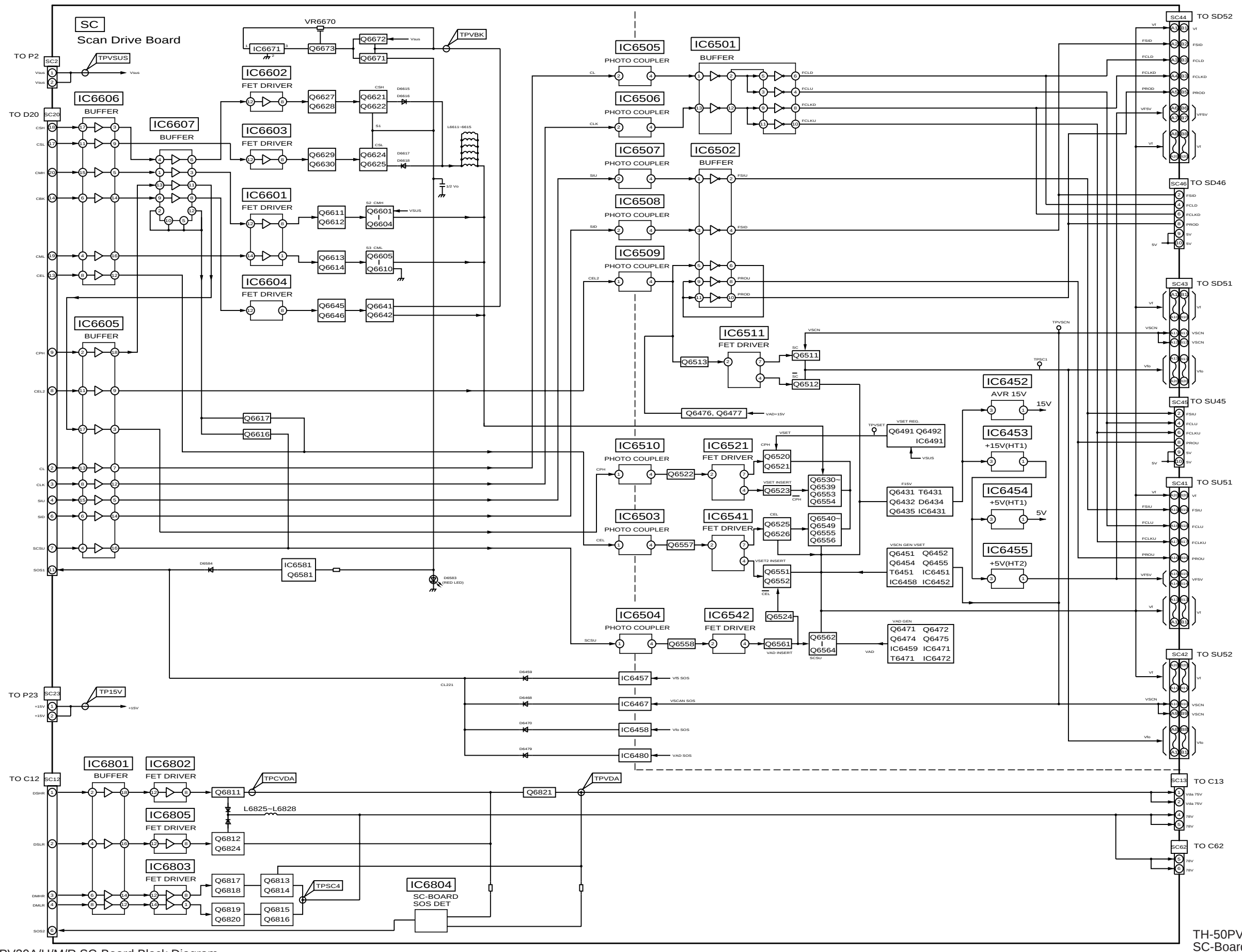
TH-50PV30A/H/M/R SC-Board Block Diagram
