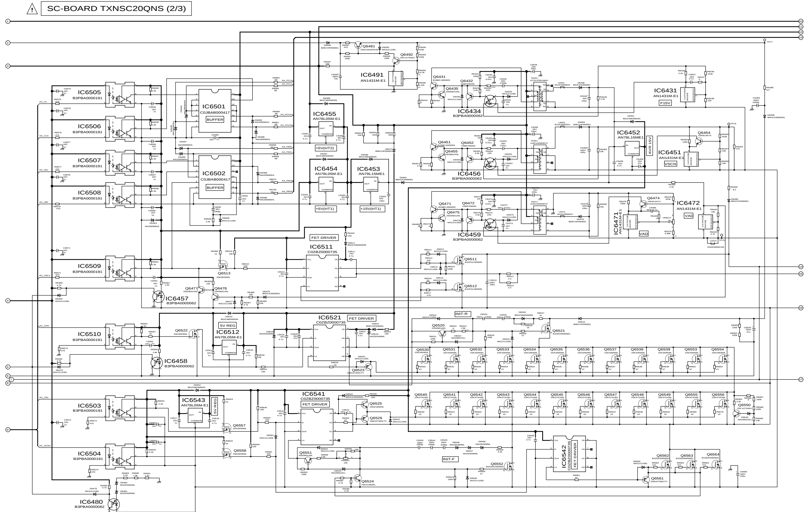
TH-50PV30A/H/M/R SC-Board (2 of 3) Schematic Diagram
