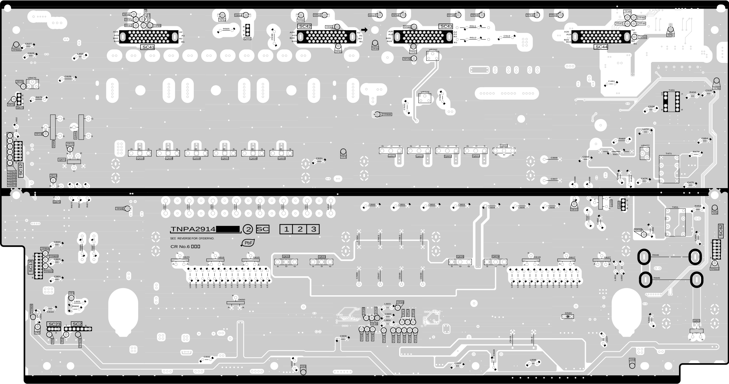
SC-BOARD (FOIL SIDE) TXNSC20QNS
