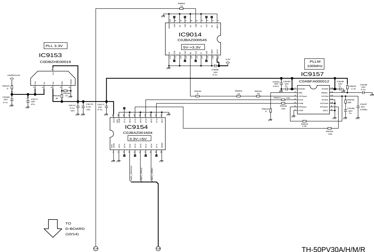
TH-50PV30A/H/M/R D-Board (4 of 14) Schematic Diagram
