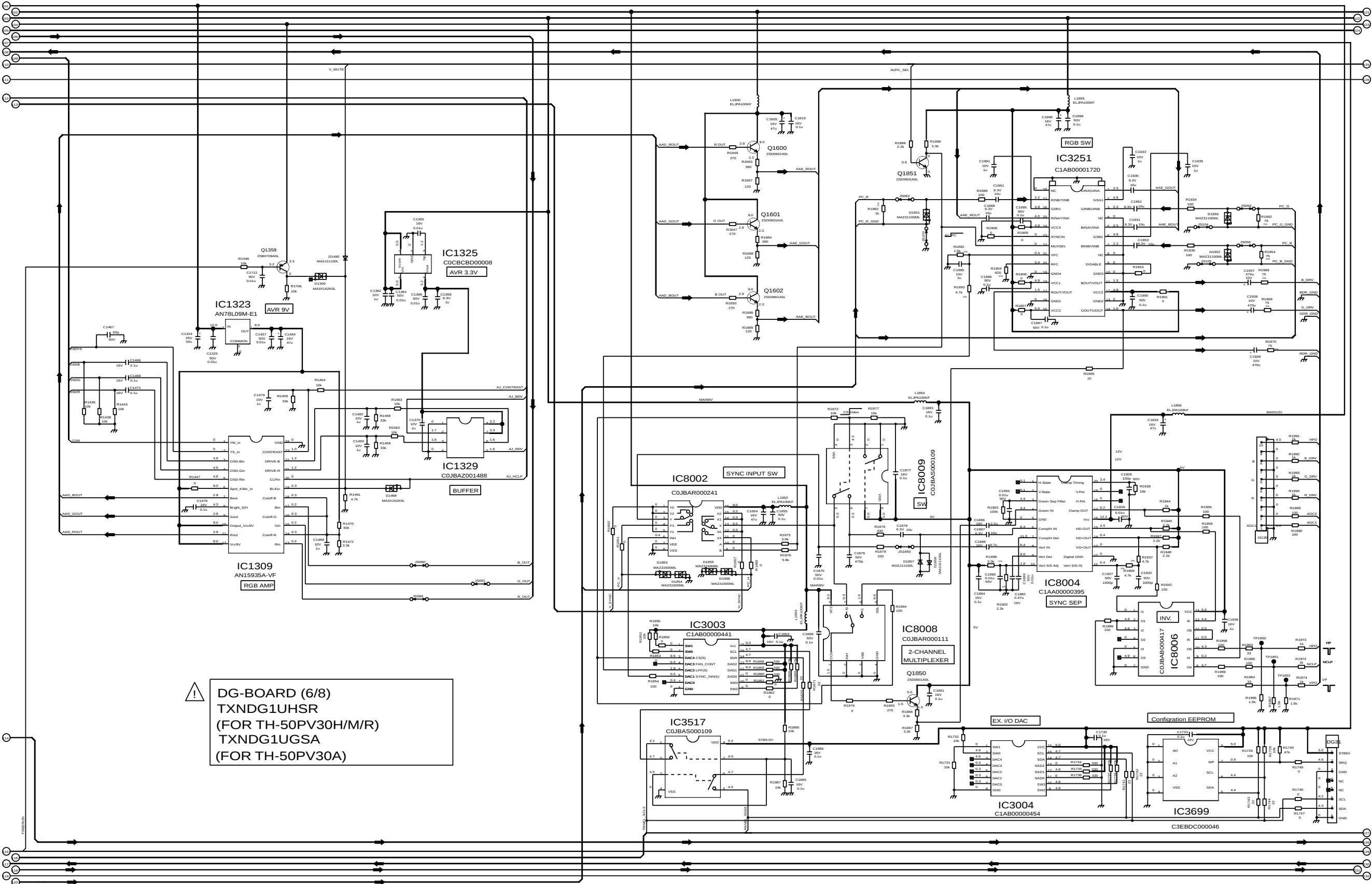
TH-50PV30A/H/M/R DG-Board (6 of 8) Schematic Diagram
