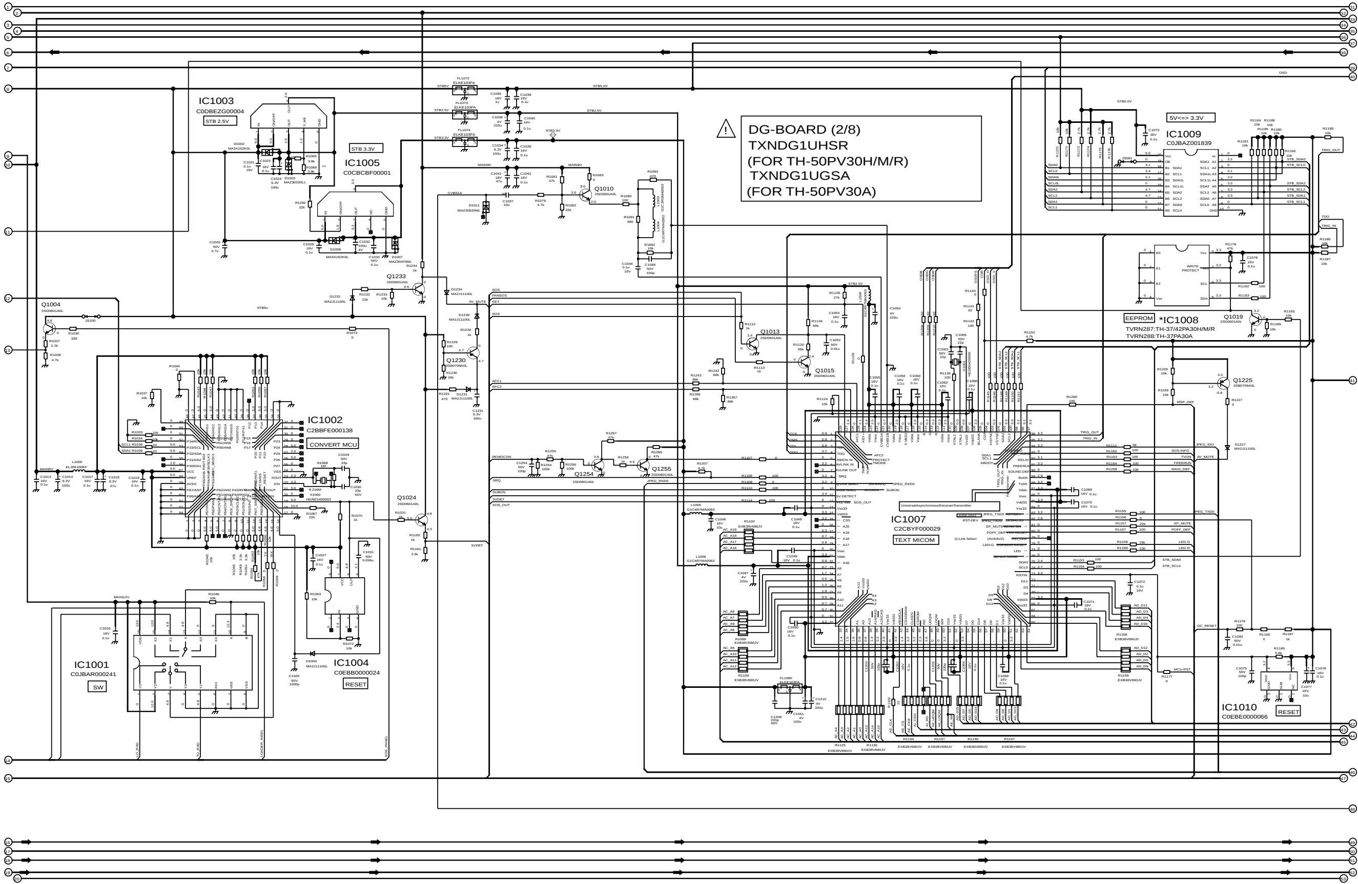
TH-50PV30A/H/M/R DG-Board (2 of 8) Schematic Diagram
