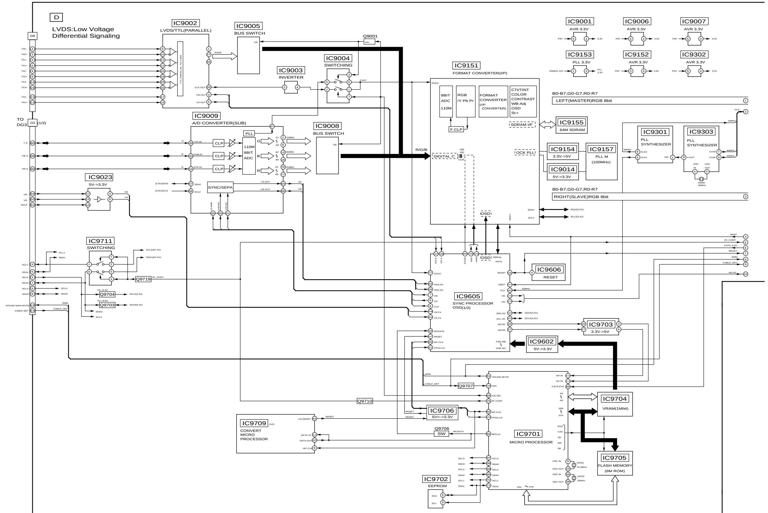
TH-50PV30A/H/M/R D-Board Block Diagram
