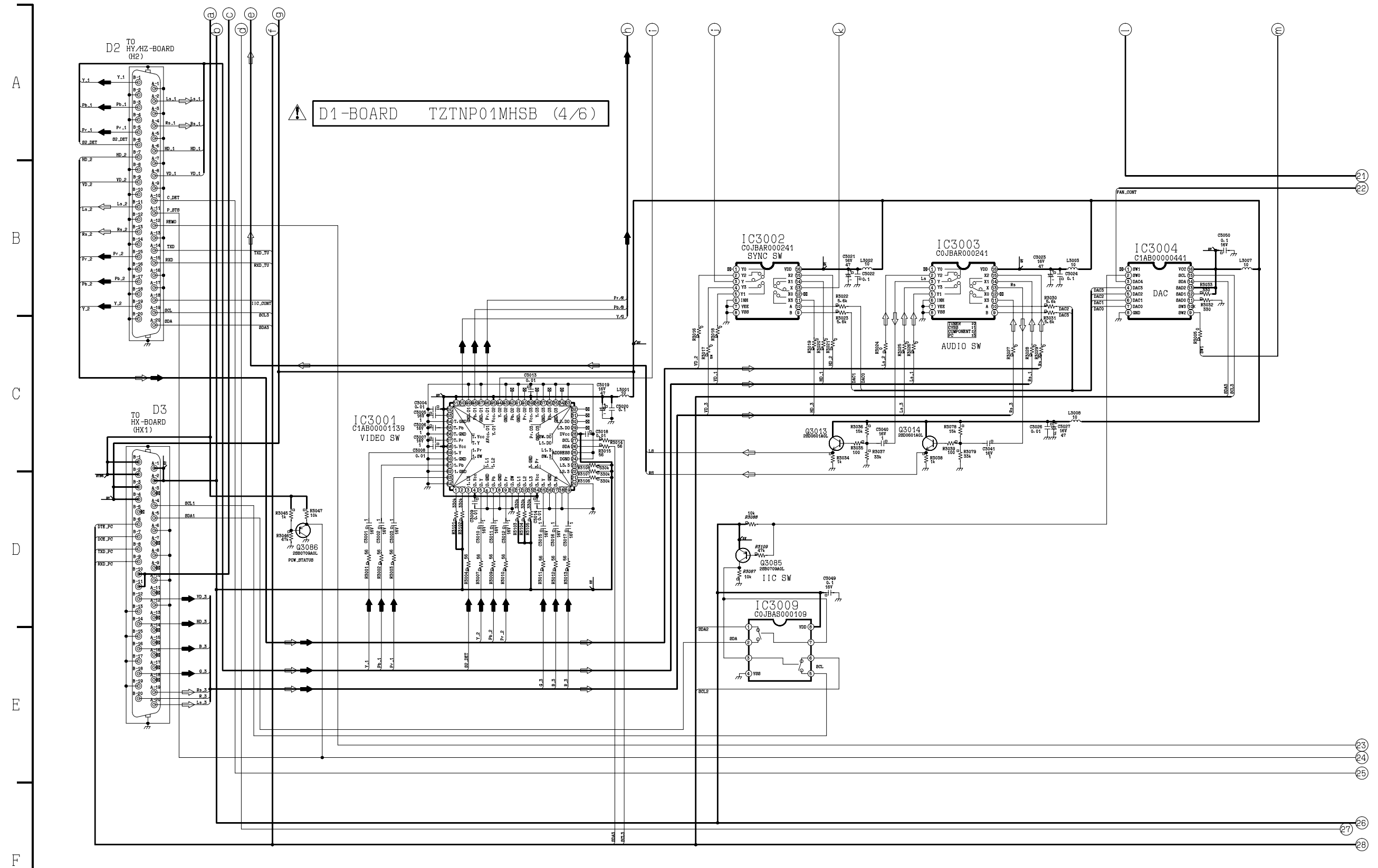
TH-50PHD5/TH-50PHW5 D1-Board (4 of 6) Schematic Diagram
