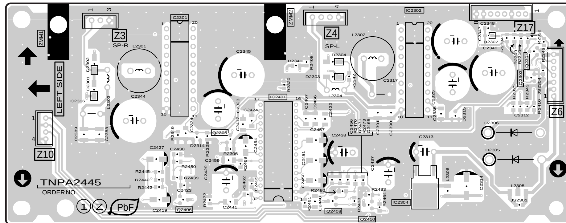
Z-BOARD (COMPONENT SIDE) TNPA2445
