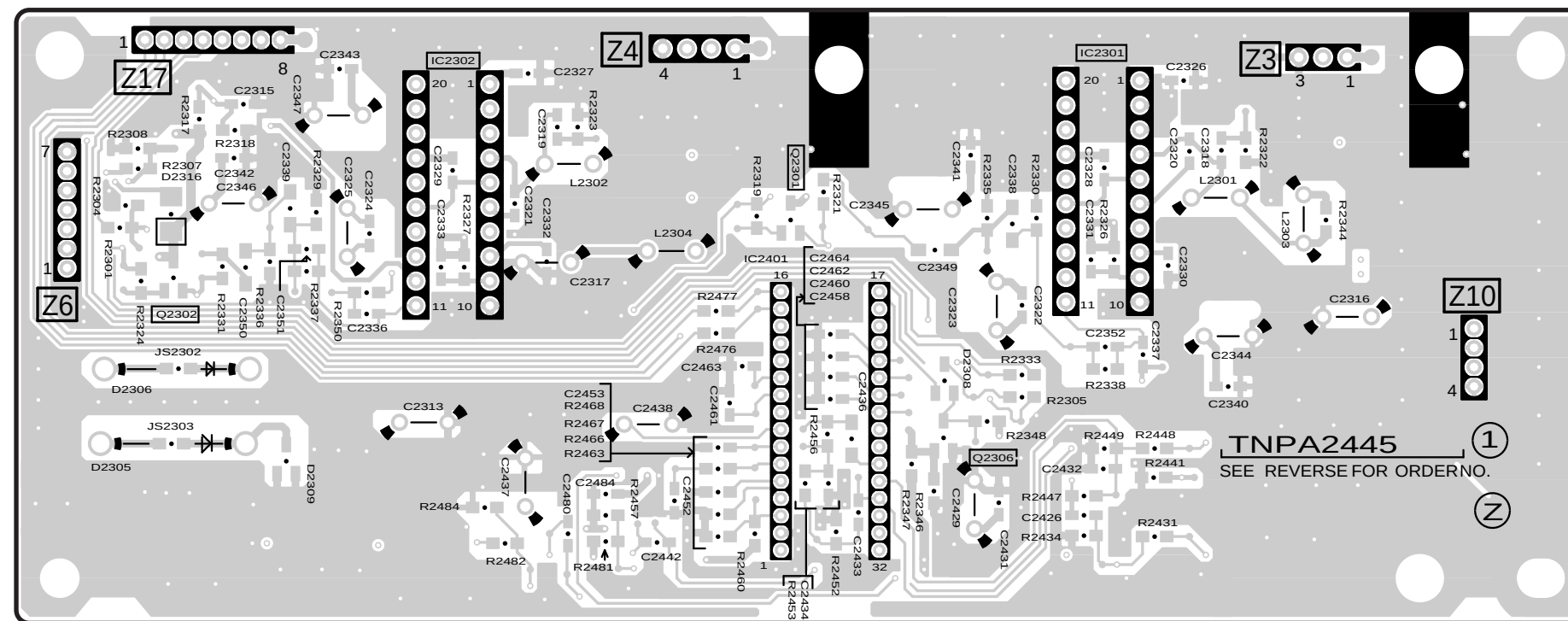
Z-BOARD (FOIL SIDE) TNPA2445
