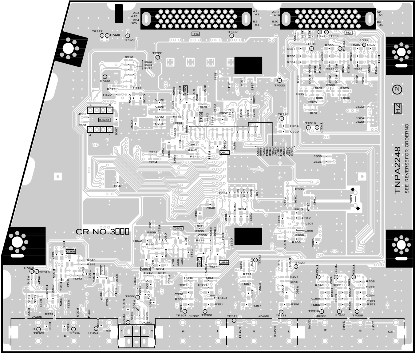
HZ-BOARD(FOIL SIDE) TXNHZ20JJS
