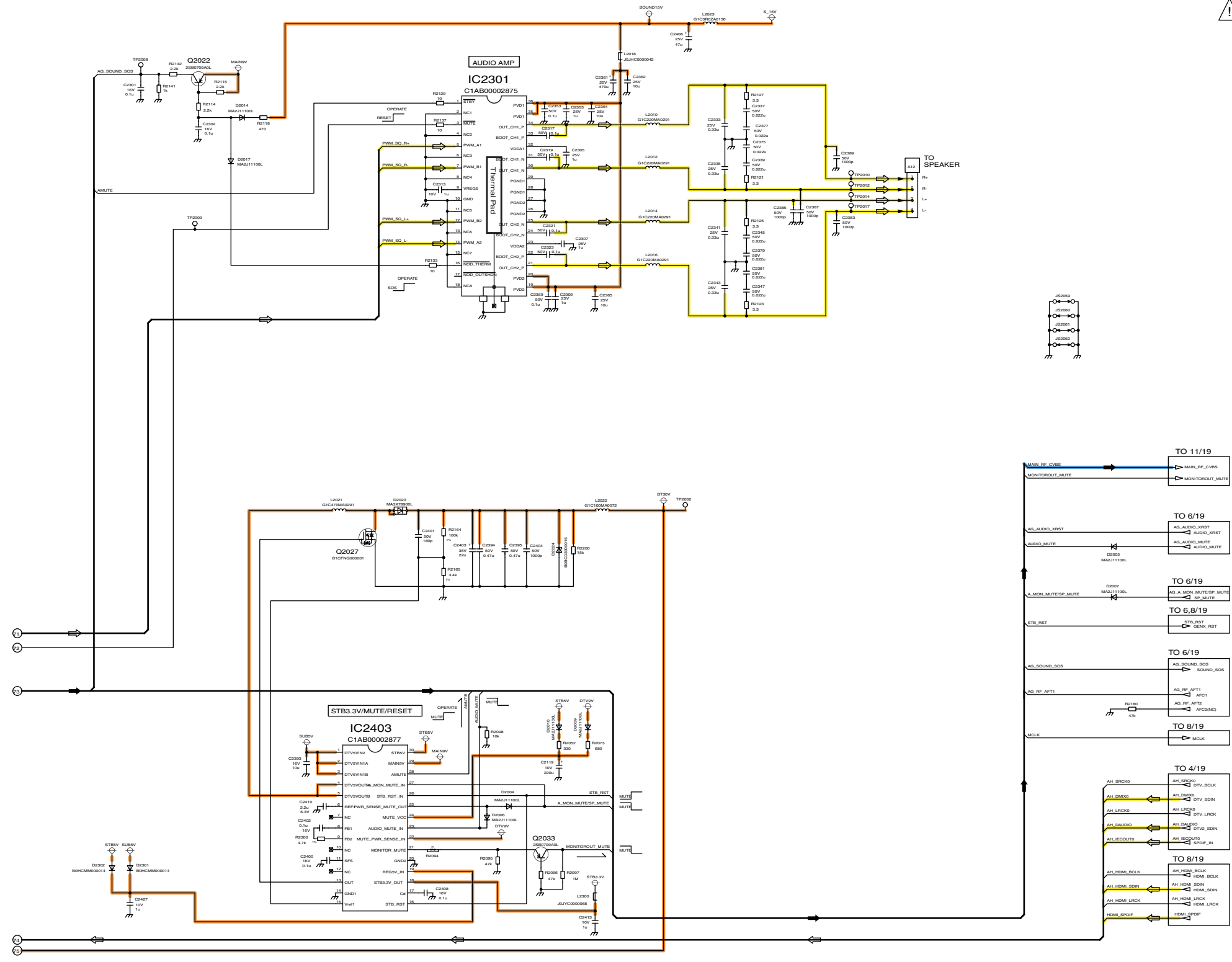
TH-42PV8D/H/HM/M/MR/MS/MT A-Board (19/19) Schematic Diagram
