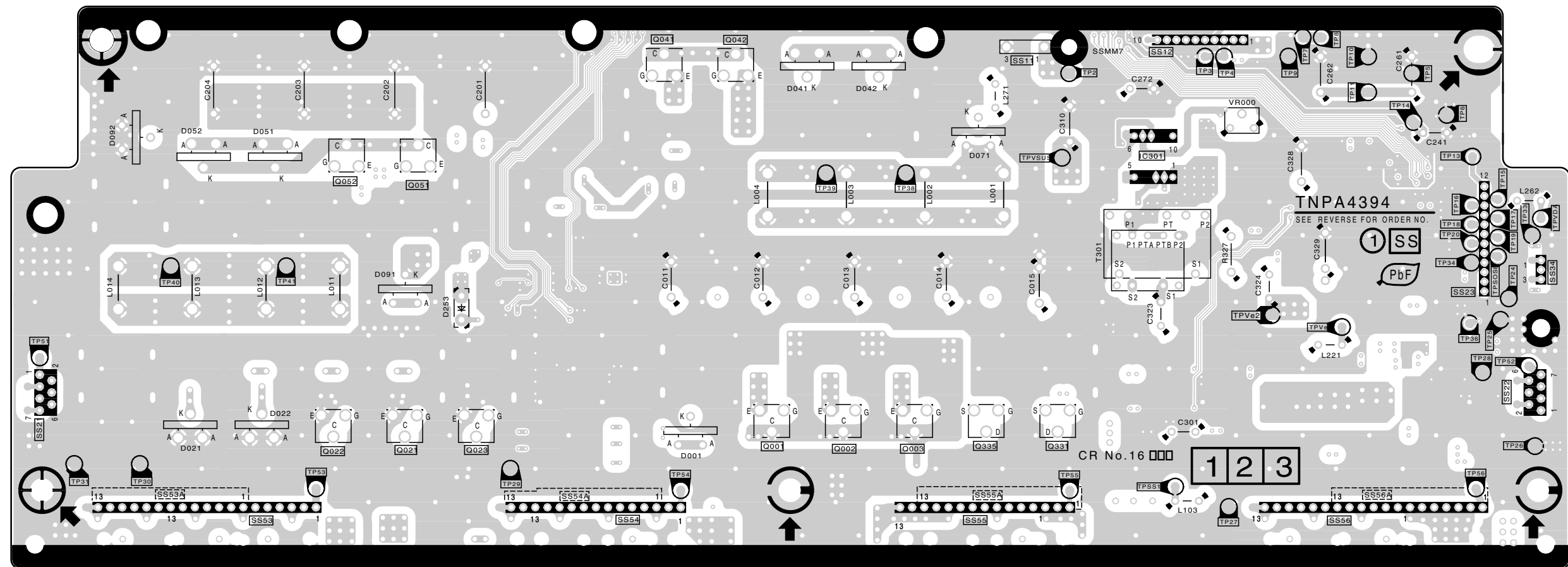
SS-BOARD (FOIL SIDE) TXNSS1RRTM
