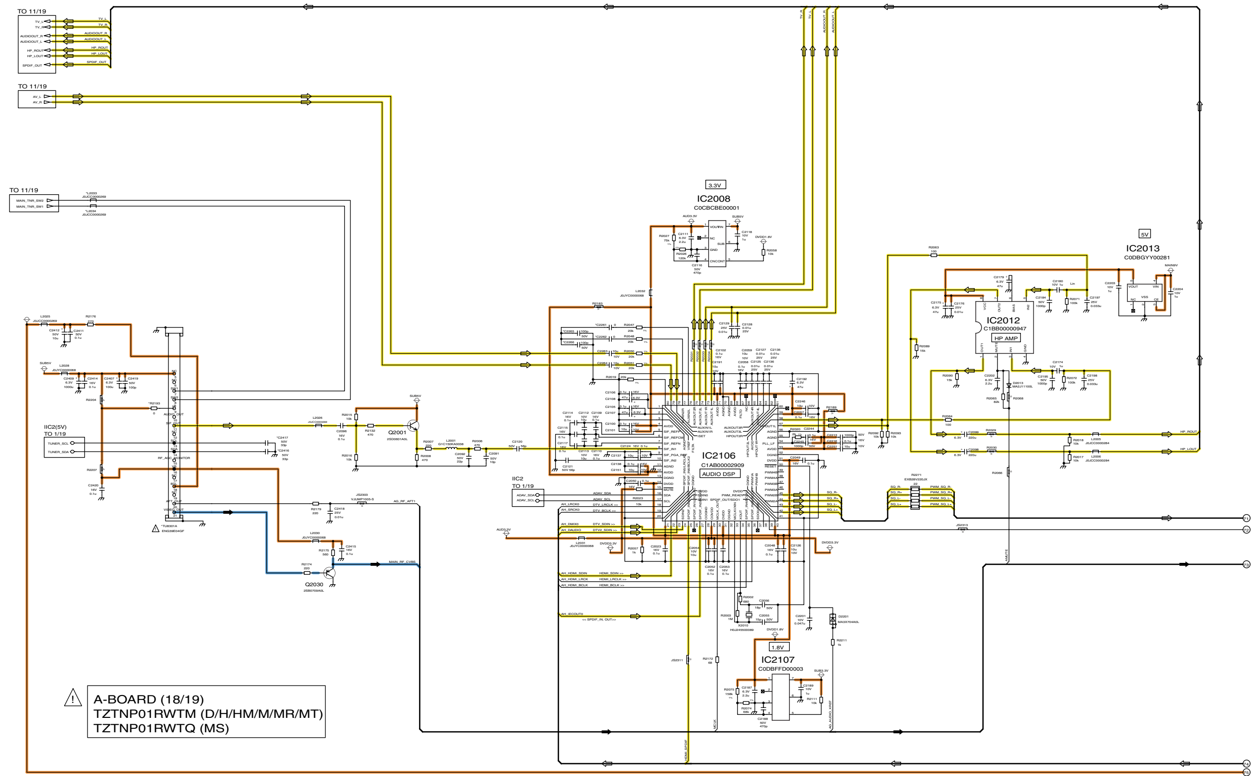
TH-42PV8D/H/HM/M/MR/MS/MT A-Board (18/19) Schematic Diagram
