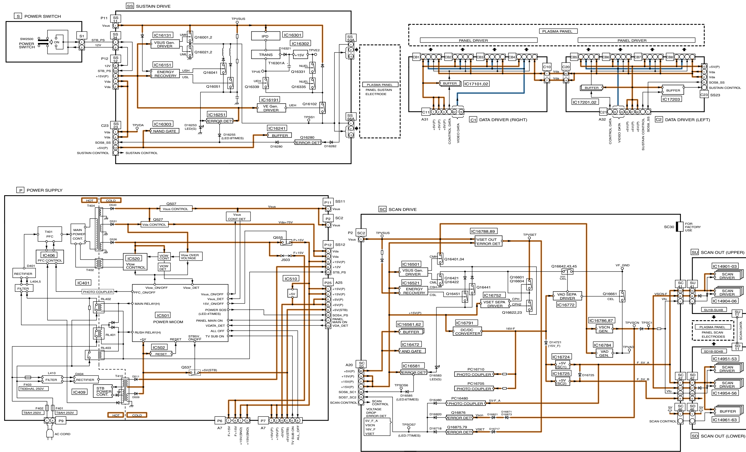
TH-42PV8D/H/HM/M/MR/MS/MT Block (5/5) Diagram
