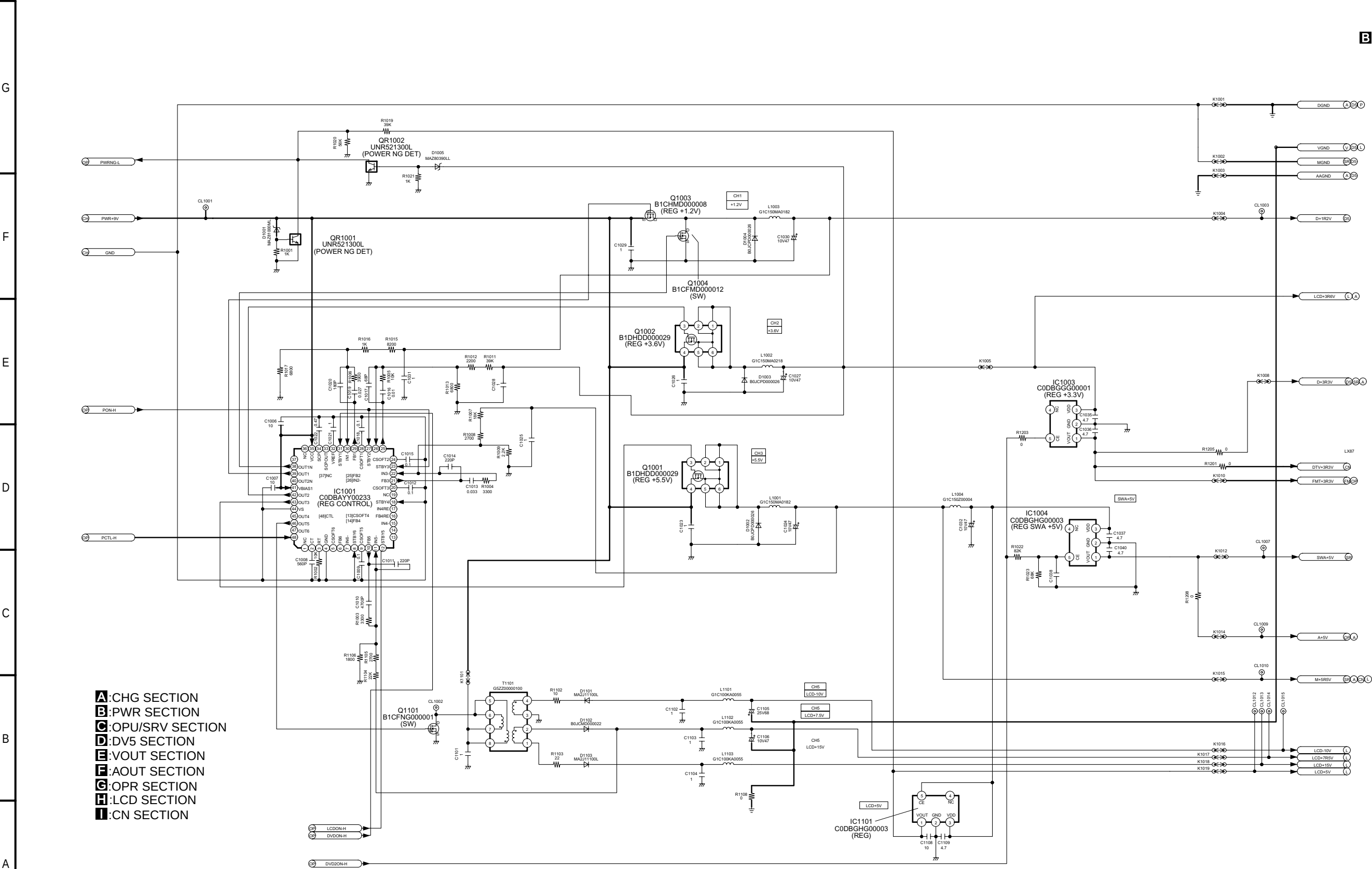
DVD-LS80EB/EG/LS82EB/EG POWER SUPPLY SECTION (MAIN P.C.B.(2/9)) SCHEMATIC DIAGRAM
