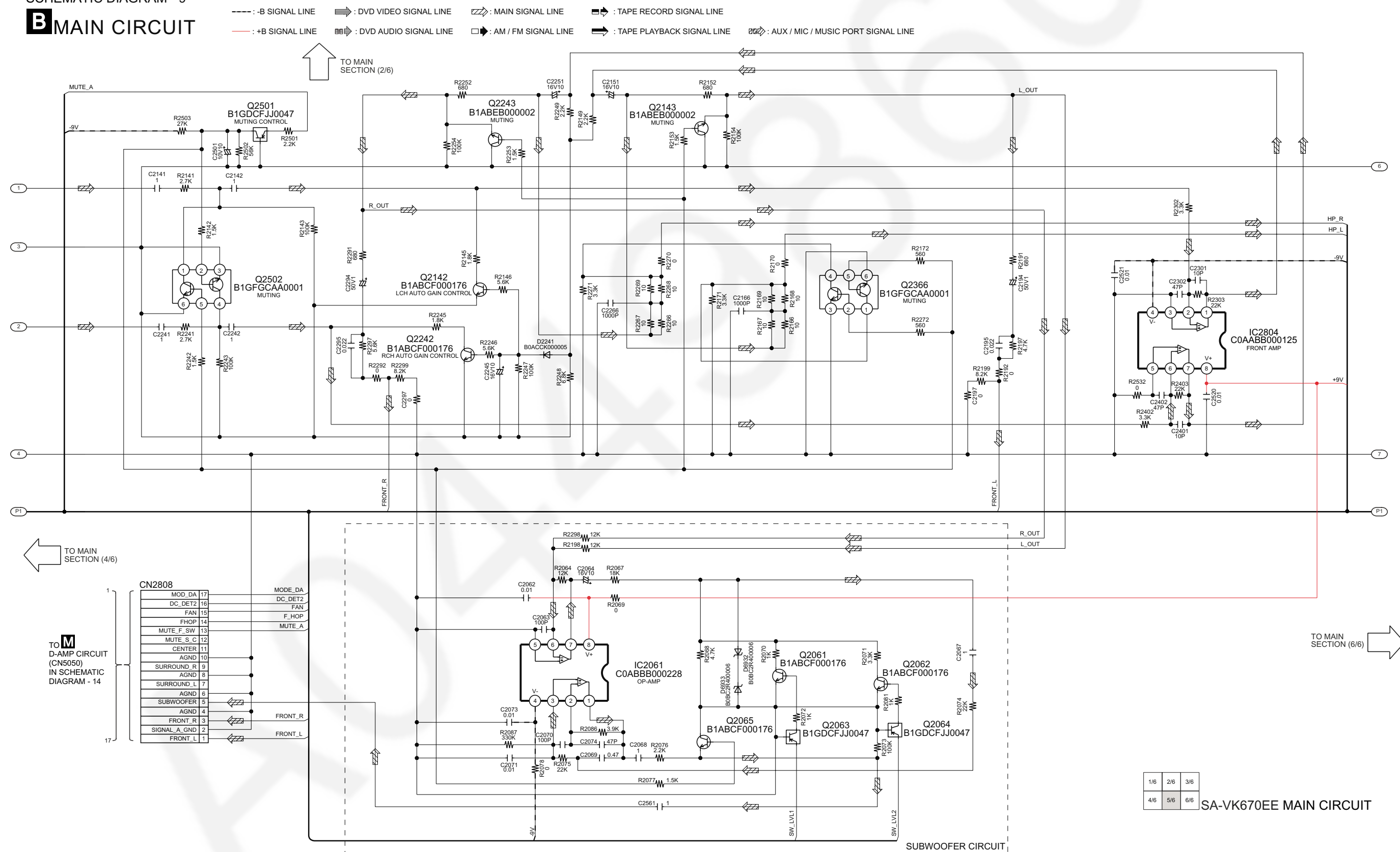
SCHEMATIC DIAGRAM - 9
