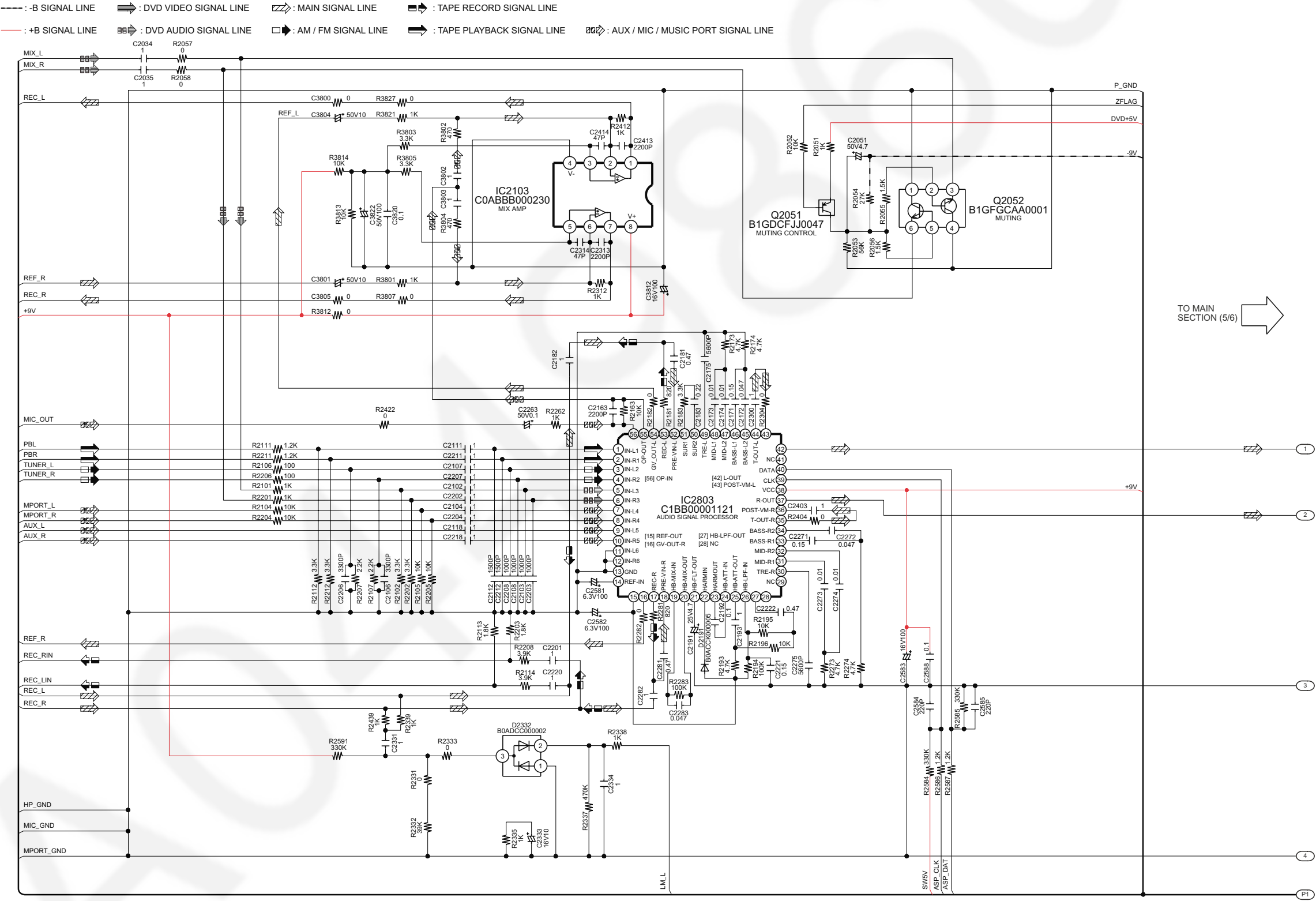
SA-VK670EE MAIN CIRCUIT
