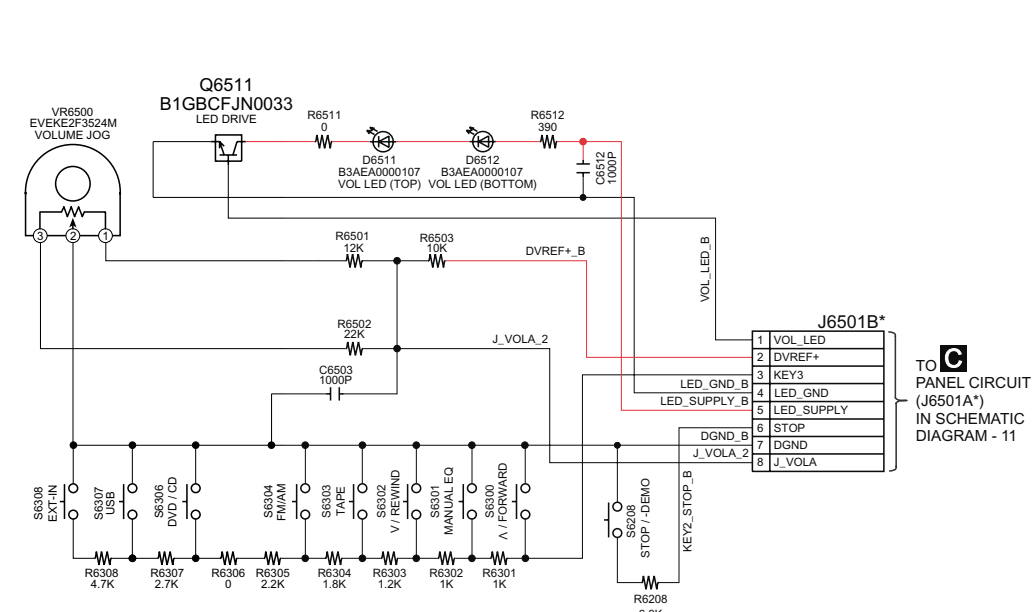
SCHEMATIC DIAGRAM - 12
