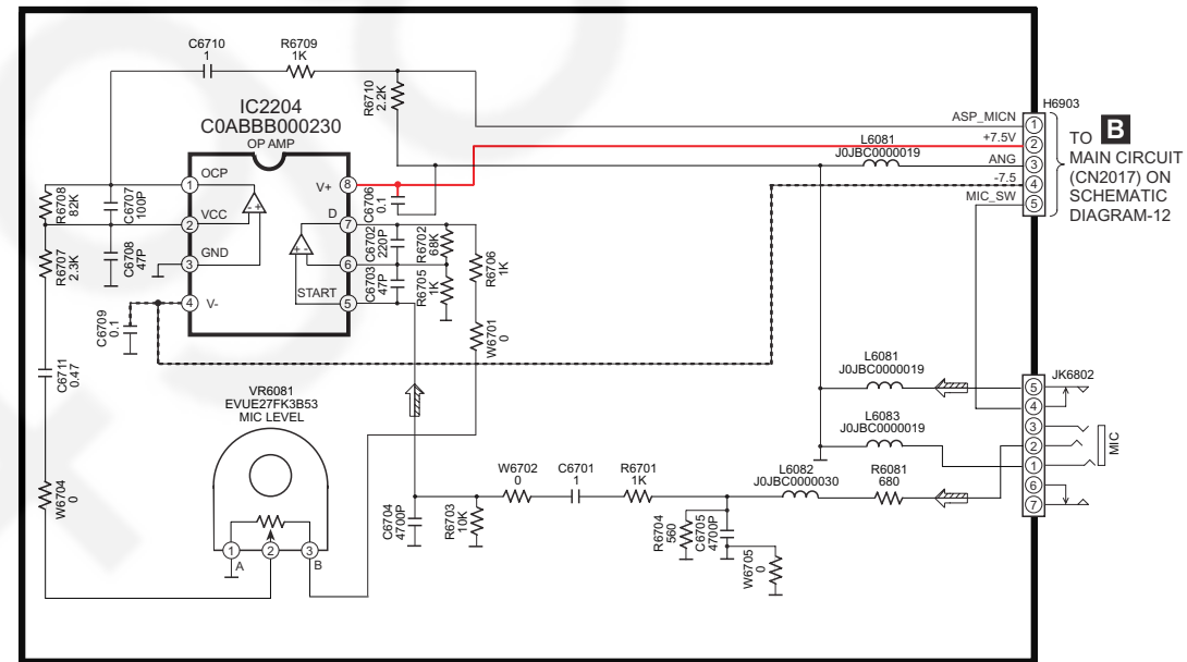
I MIC CIRCUIT
