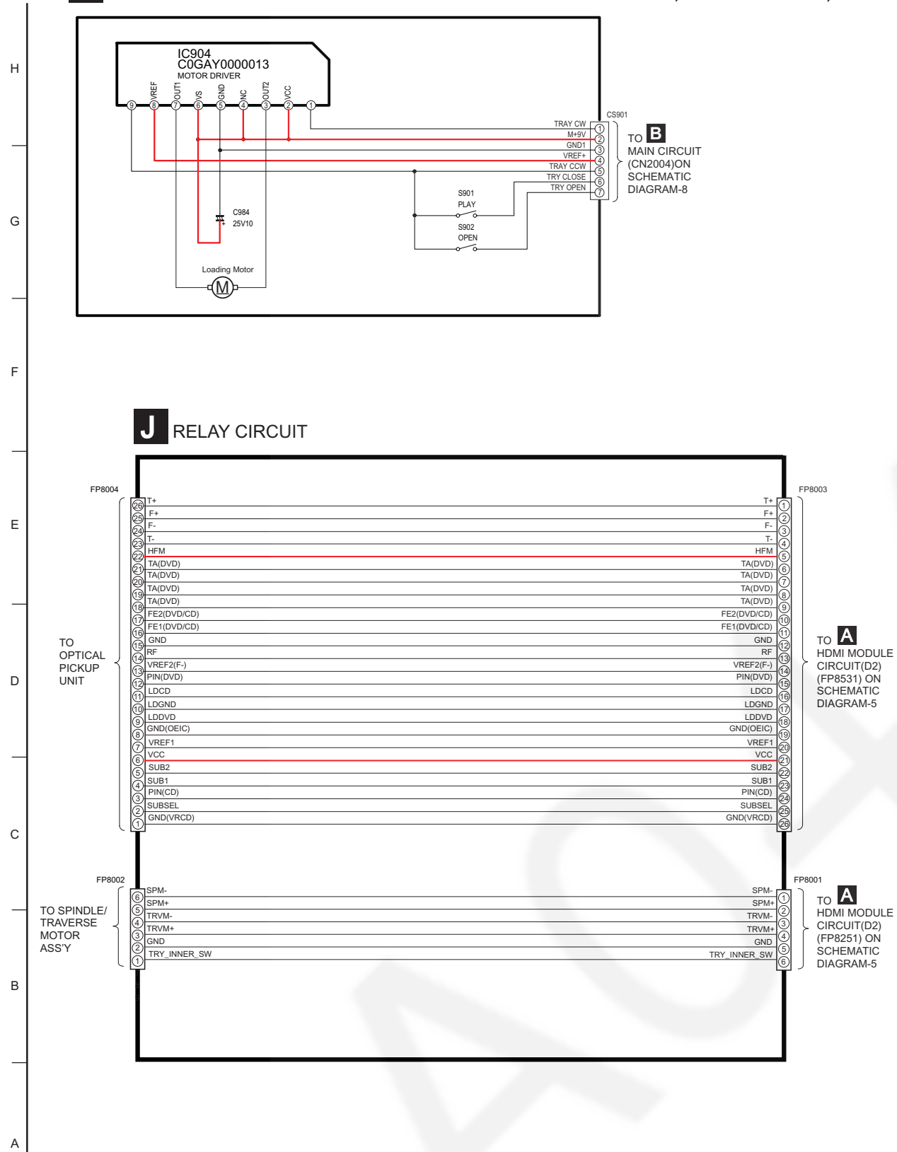
SCHEMATIC DIAGRAM-18
