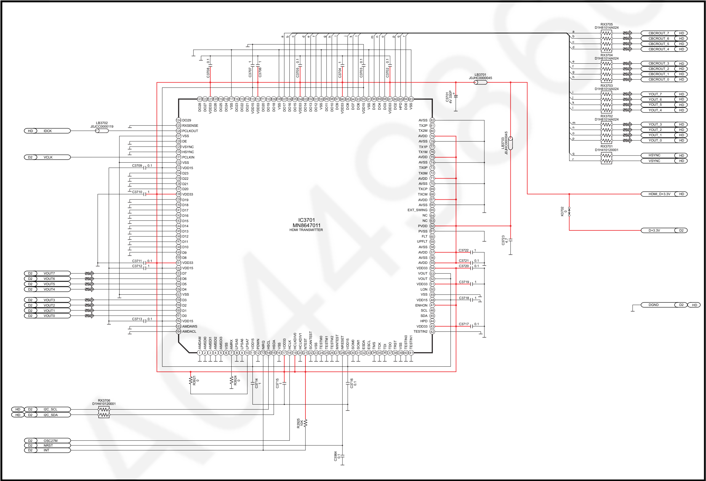
SA-HT895EE HDMI MODULE CIRCUIT (UP)
