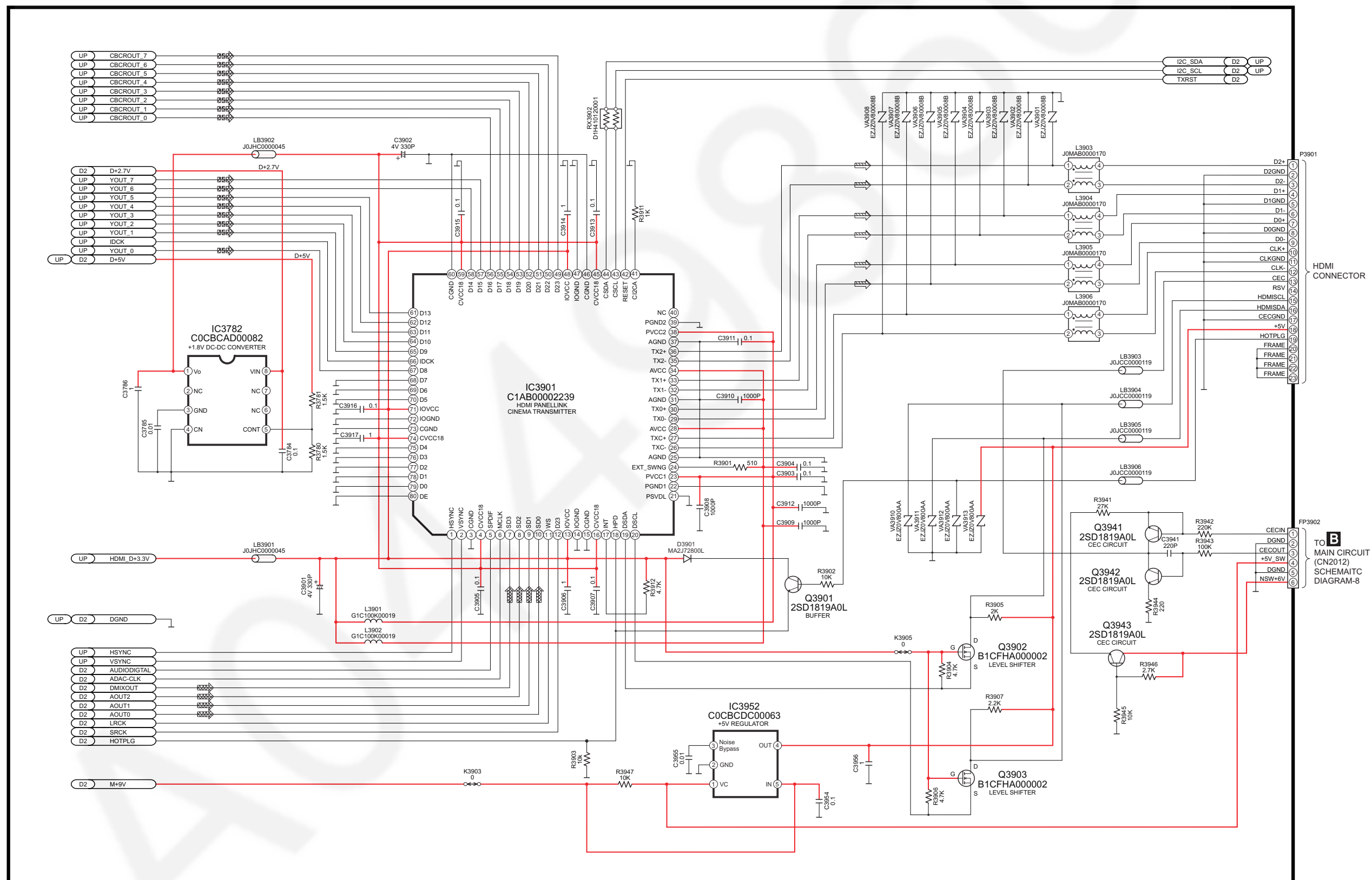
SA-HT895EE HDMI MODULE CIRCUIT
