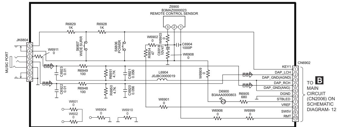
F MUSIC PORT CIRCUIT
