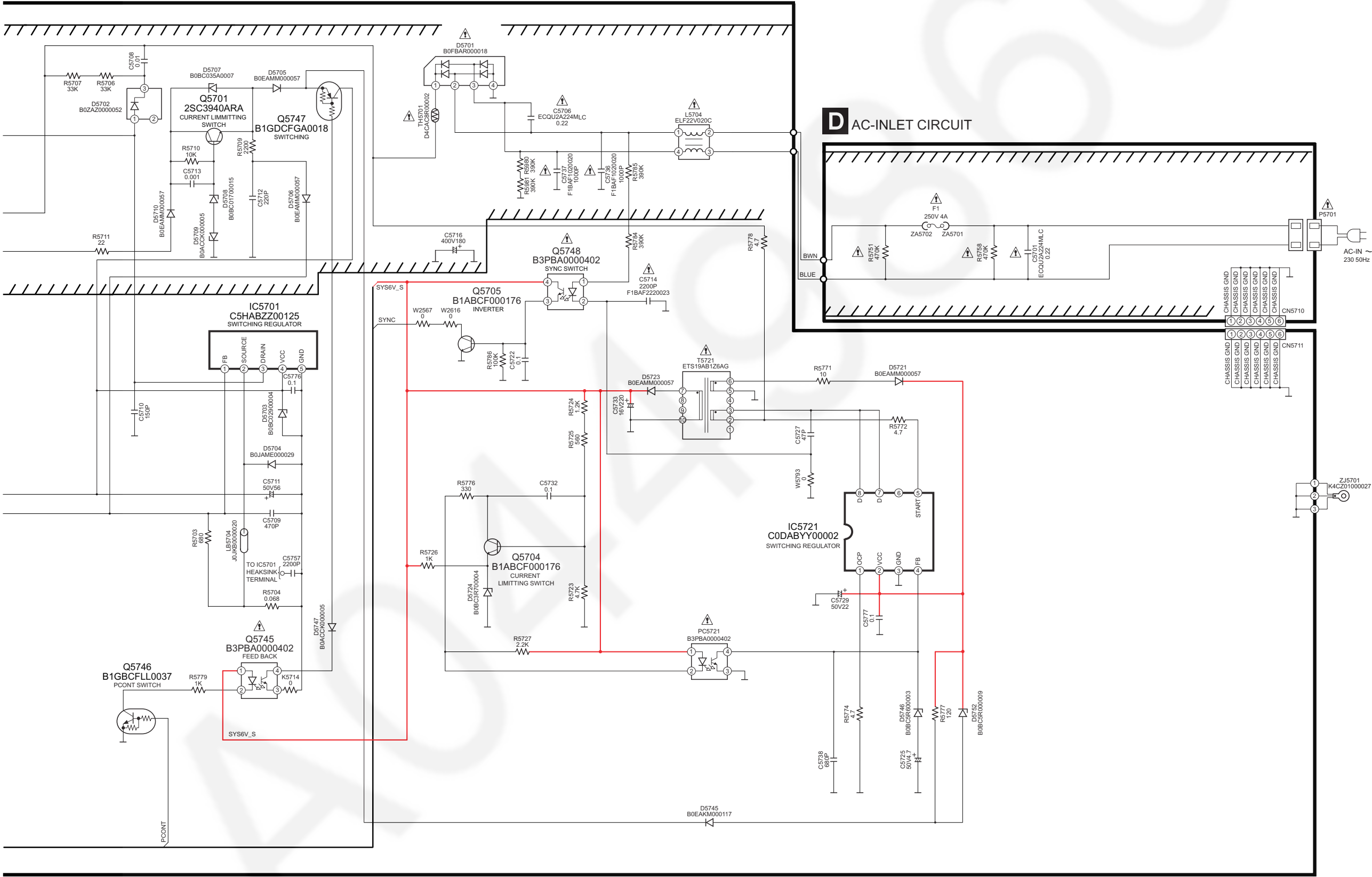
SA-HT895EE POWER(SMPS)/AC-INLET CIRCUIT
