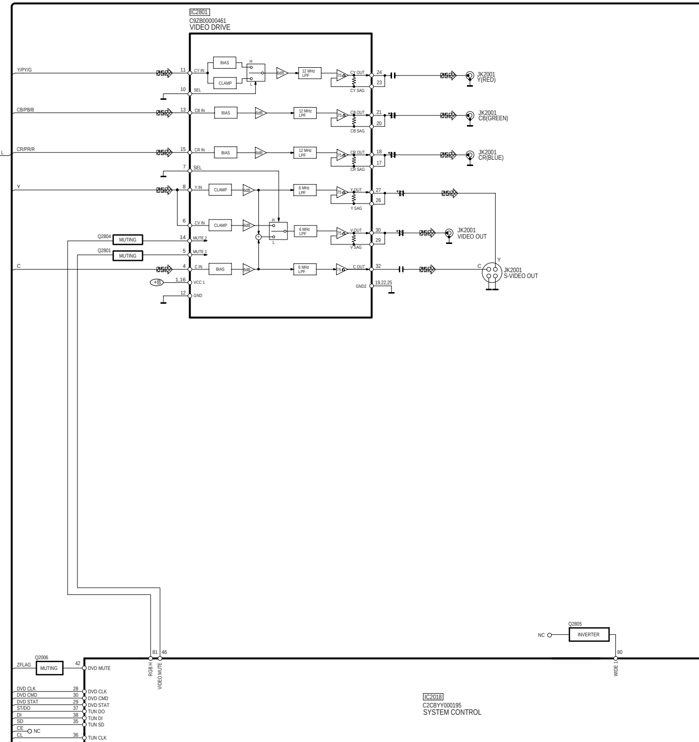
SA-HT540GC/GCS/GCT/GS BLOCK DIAGRAM
