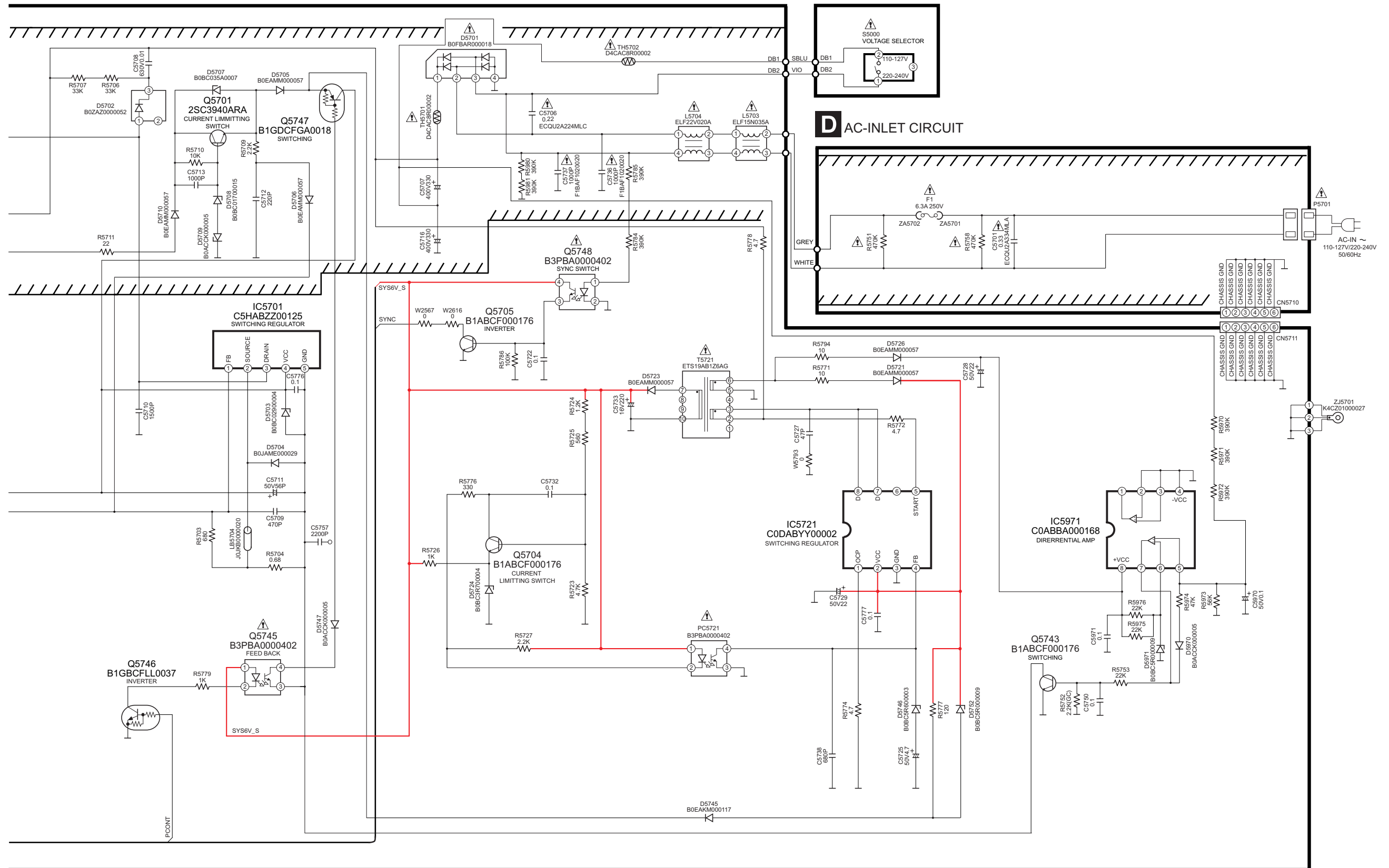
SA-HT540GC/GS/GCS/GCT POWER(SMPS)/ AC INLET/ VOLTAGE SELECTOR CIRCUIT
