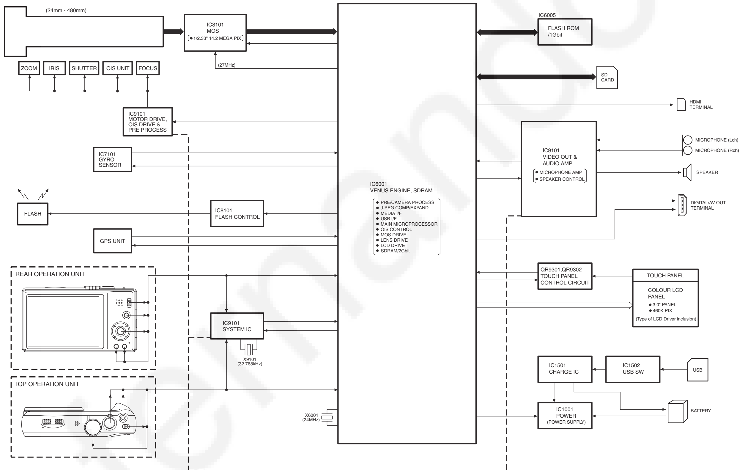
DMC-TZ27/TZ30/TZ31, ZS19/ZS20 OVERALL BLOCK DIAGRAM
