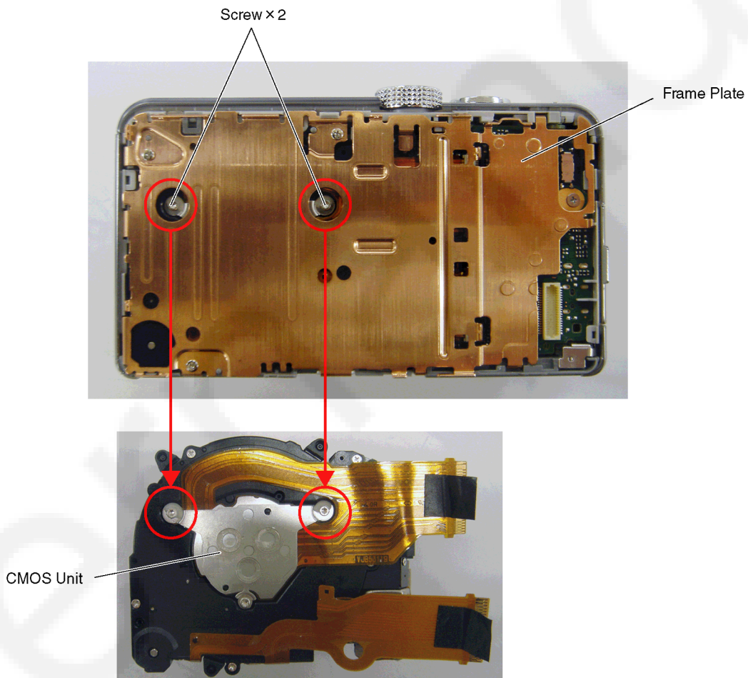
The Optical tilt adjustment can be performed with the Frame Plate attached
