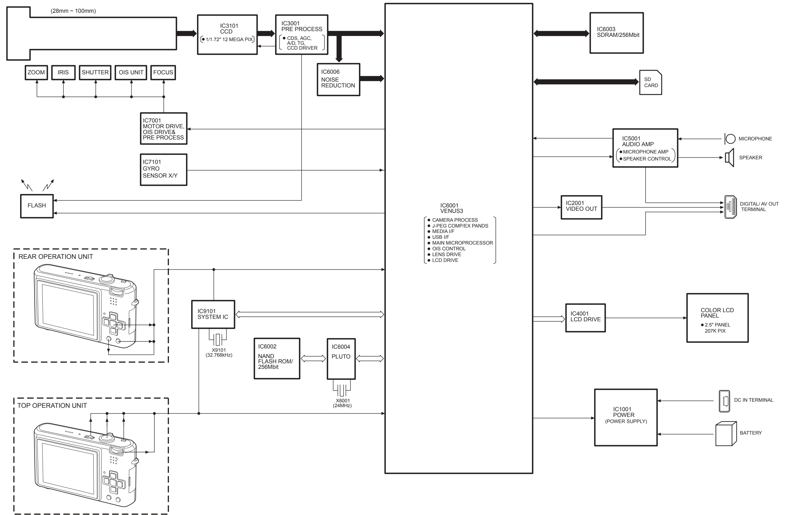
DMC-FX100 OVERALL BLOCK DIAGRAM
