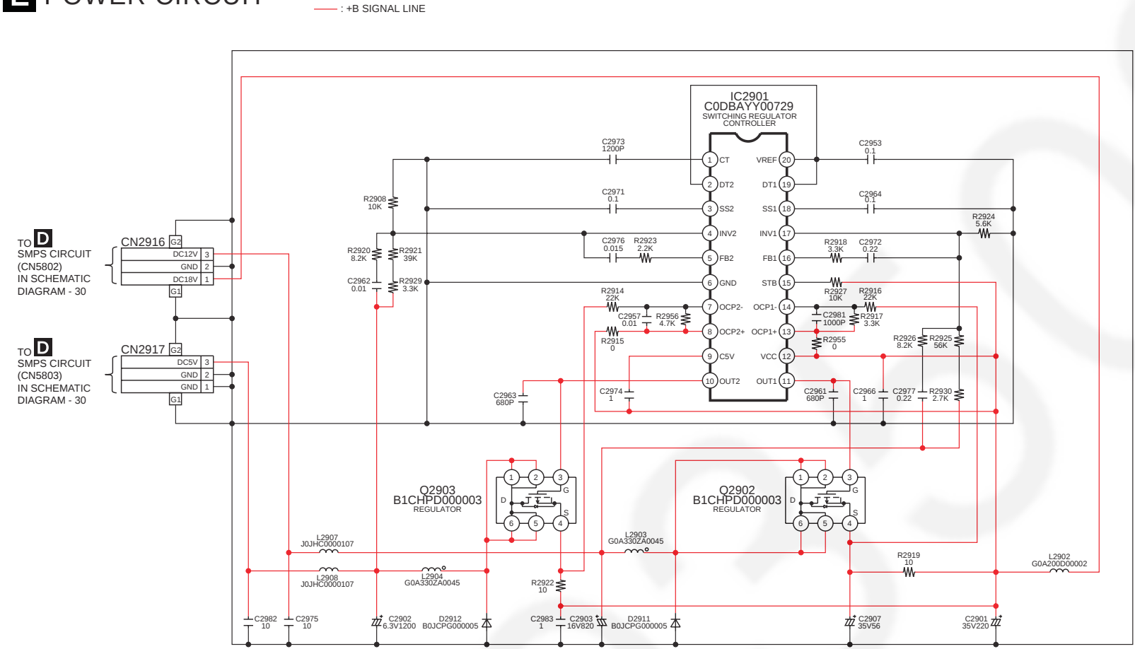
SCHEMATIC DIAGRAM - 32
